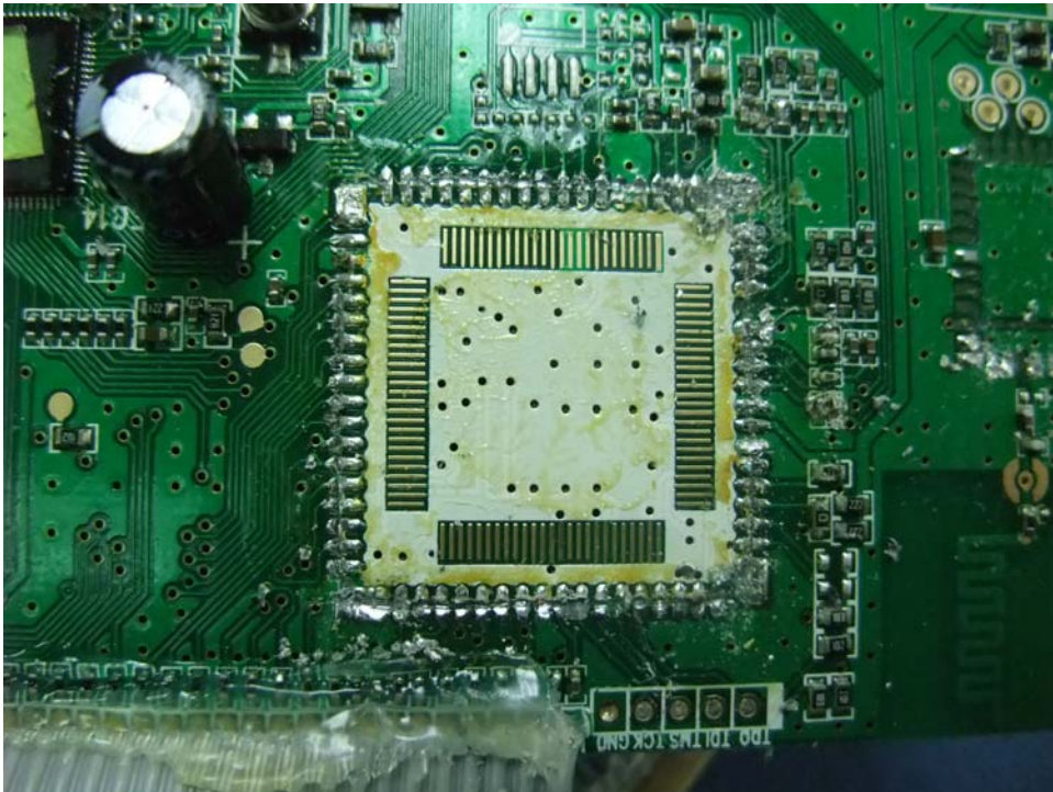
EUT Main PCB comp side (View 3)
