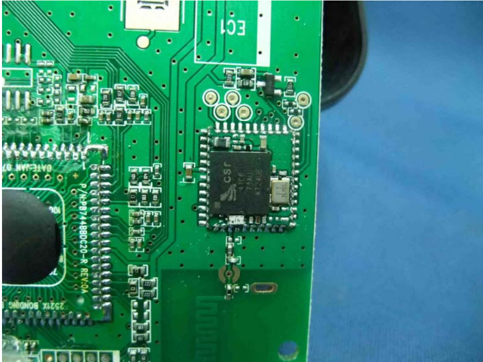
EUT Main PCB comp side (View 4)
