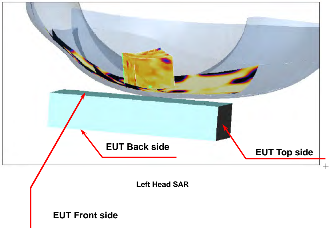
Figure 4. Left Head SAR Test Setup (Cheek)
