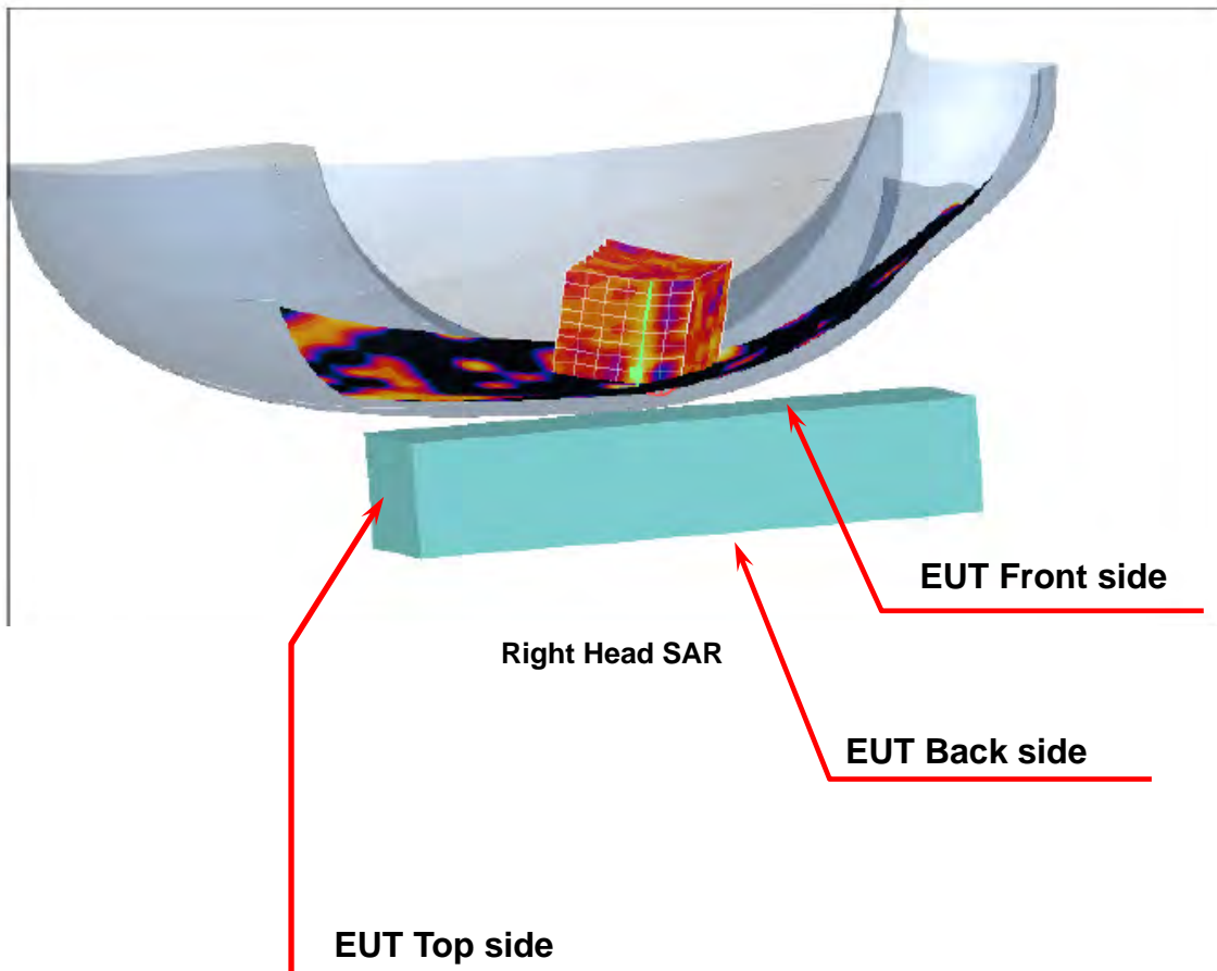
Figure 2. Right Head SAR Test Setup (Cheek)
