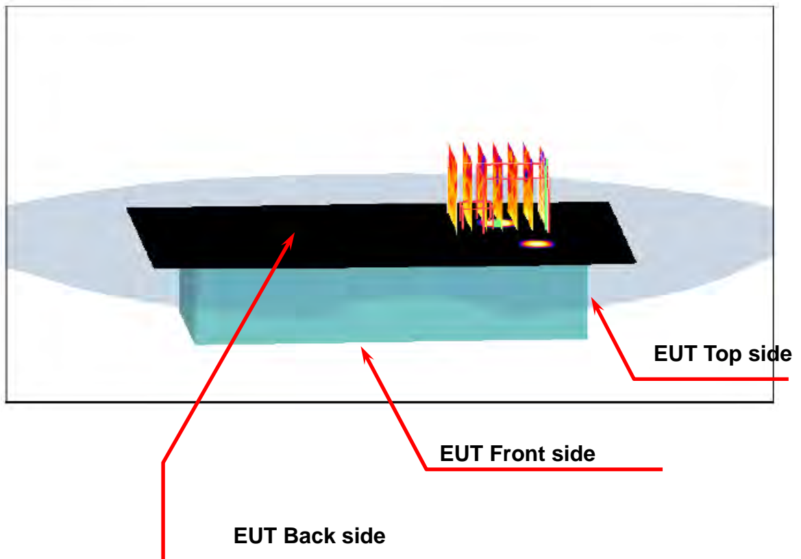
Figure 6. Body SAR Test Setup (Flat Section)
