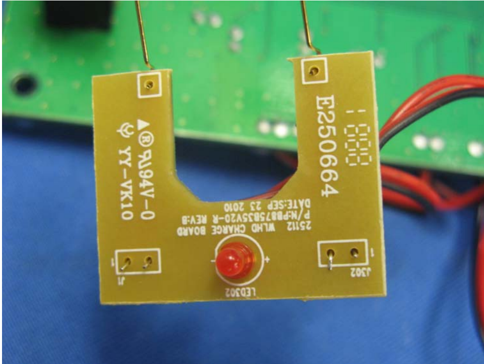
Base Unit Charge Board front side
