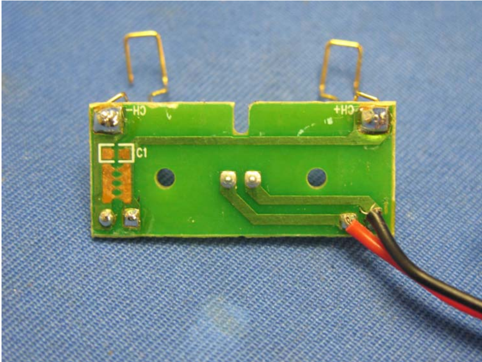
Base Unit another Charge Board rear side
