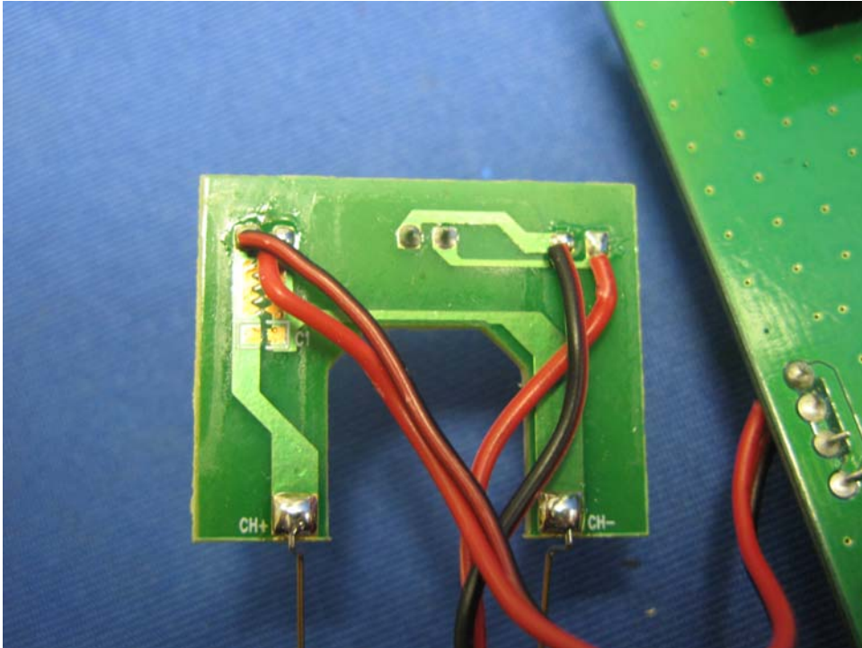
Base Unit Charge Board rear side (View 2)
