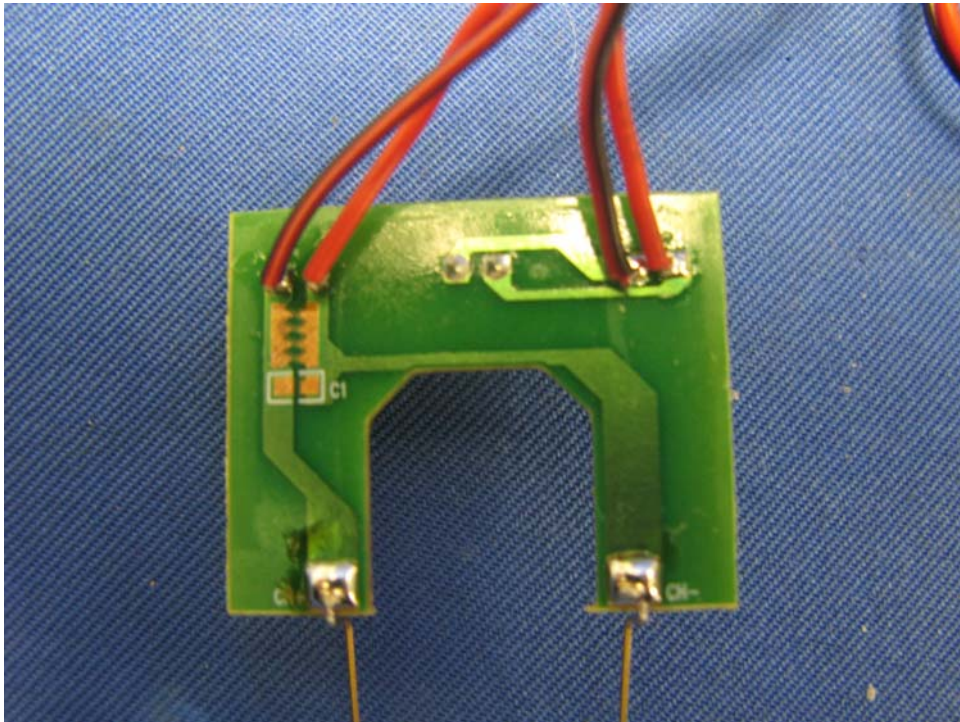
Base Unit Charge Board rear side (View 1)
