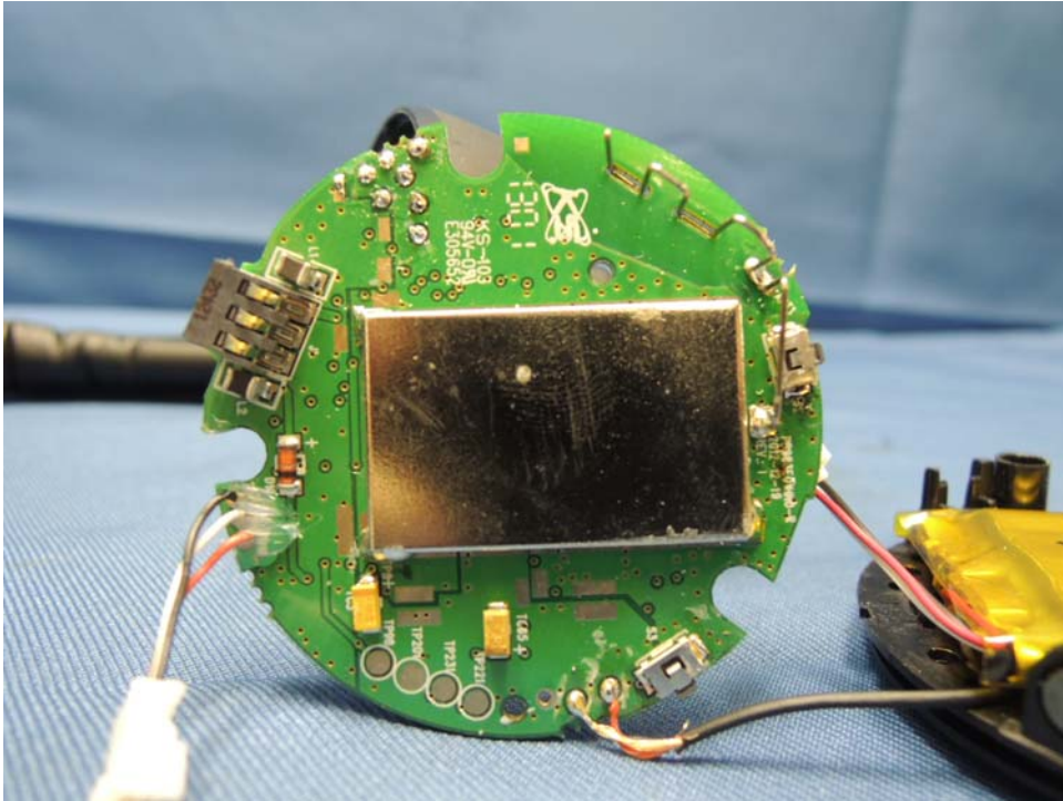
Headphone Main PCB comp side
