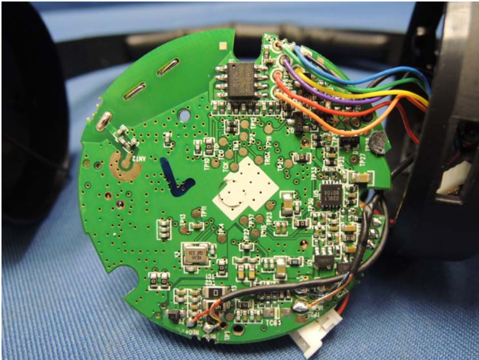
Headphone Main PCB solder side
