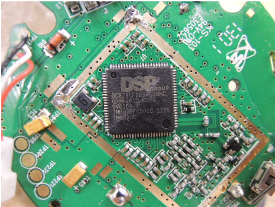
Headphone Oscillator PCB comp side
