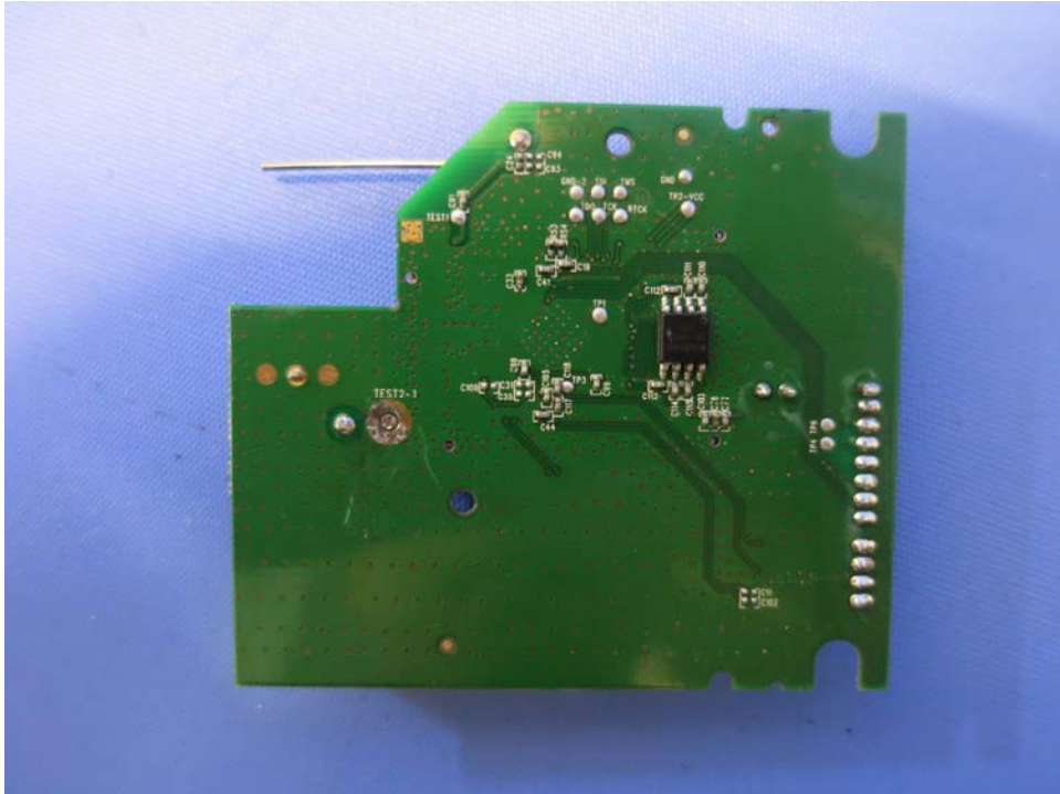
External RF module Main PCB solder side
