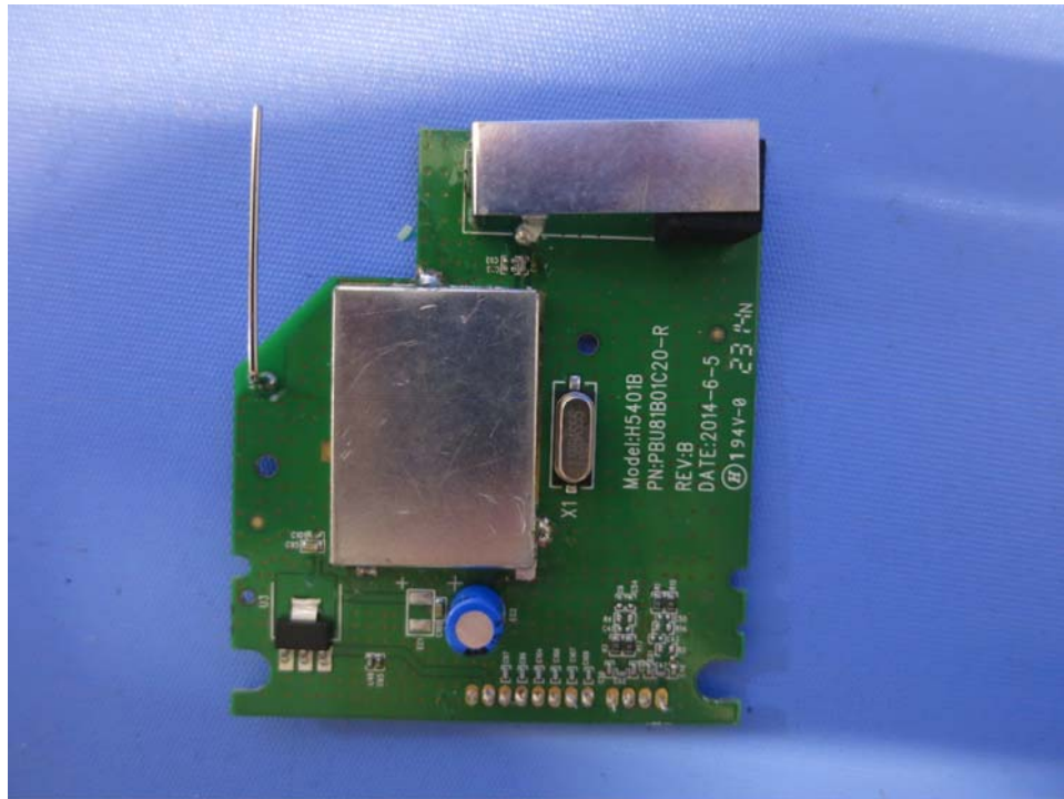
External RF module Main PCB comp side (View 1)
