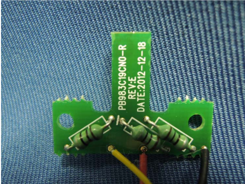
Base Unit Charging Board rear side
