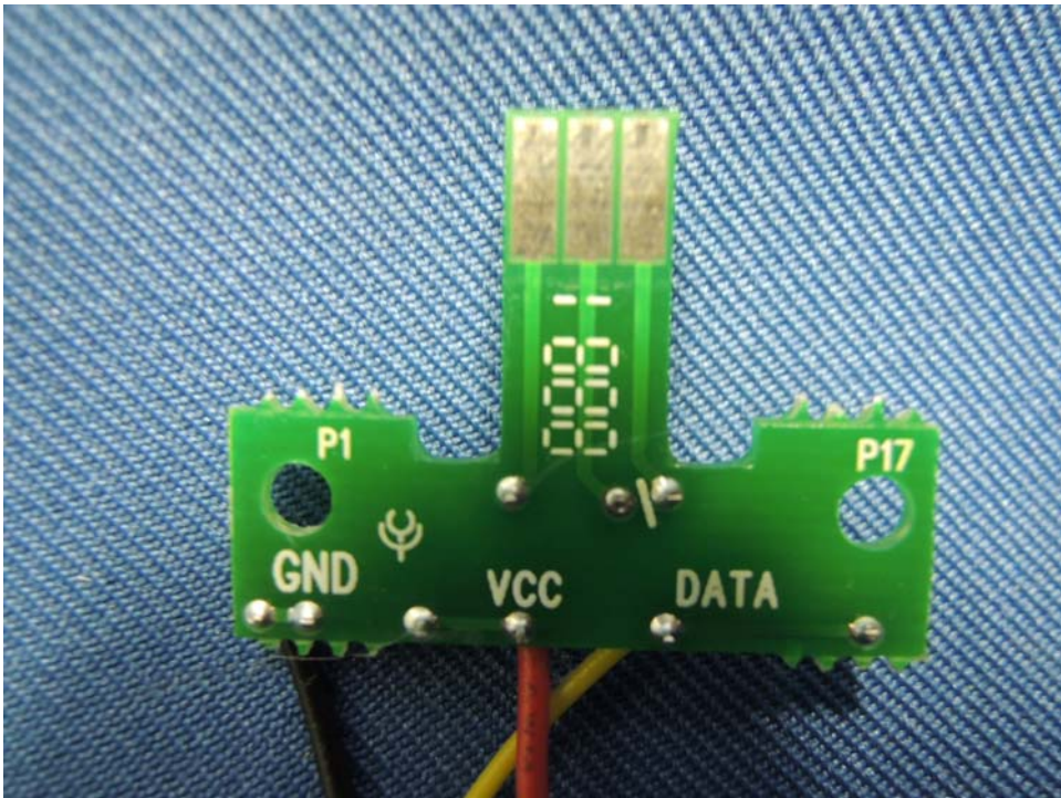
Base Unit Charging Board front side
