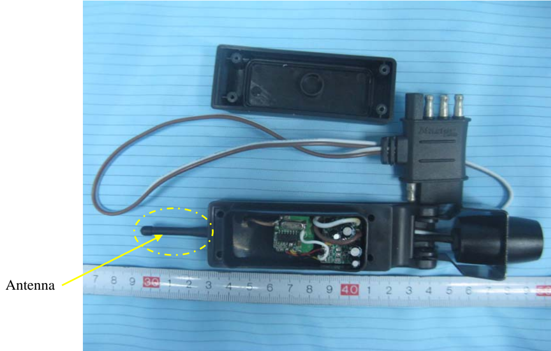
EUT - Uncovered View
