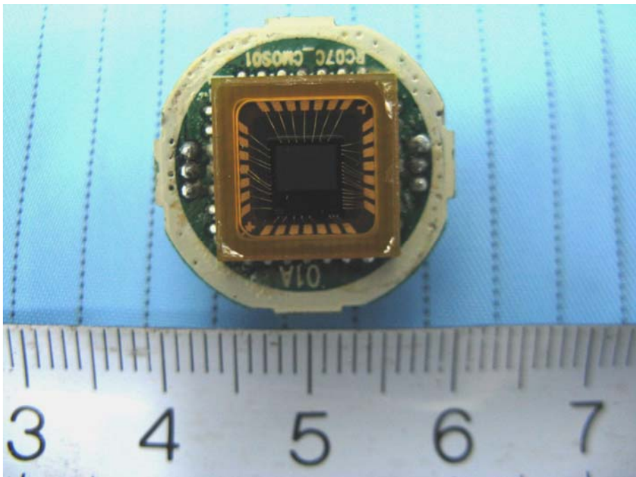
EUT - Camera Board Top Components View
