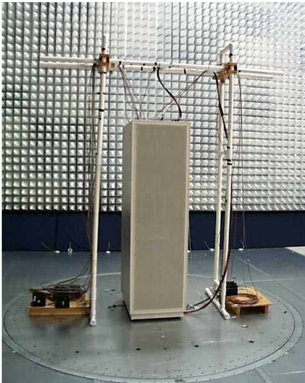
Photograph 2: Indoor Unit, rear view
