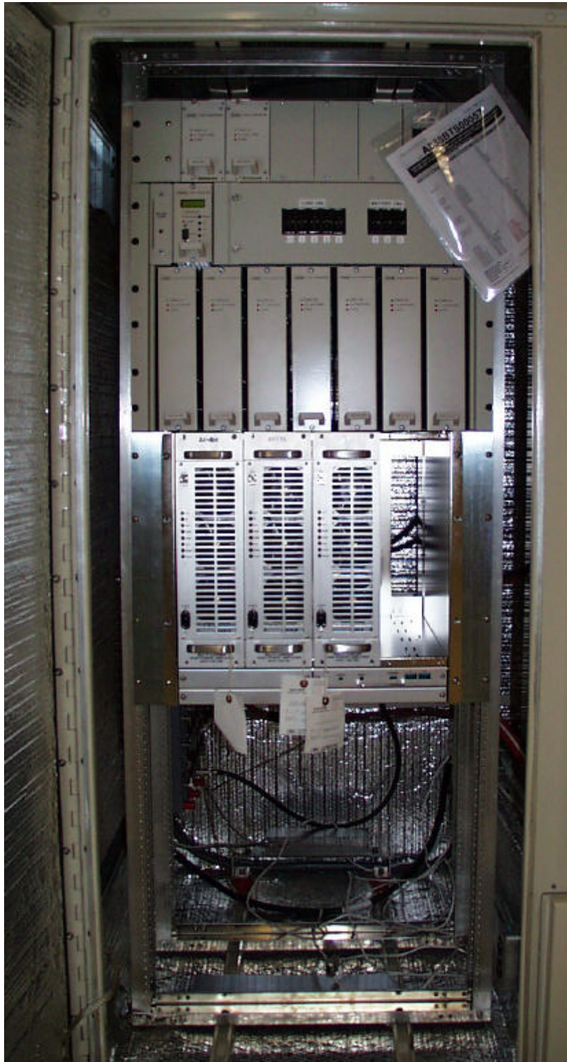
Photograph 4: Outdoor Enclosure – Front view door open, left side
