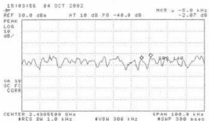
Figure 6.6(a) Spectral Density (low channel) (top) Spectrum Scan, (mid) Spectral Density, (bottom) Line Spacing. HA2401-AGC1000 Amplifier (1000 mW)
