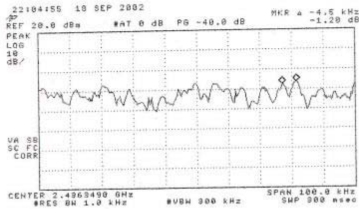
Figure 6.5(b) Spectral Density (high channel) (top) Spectrum Scan, (mid) Spectral Density, (bottom) Line Spacing. HA2401-AGC-250 Amplifier (250 mW)
