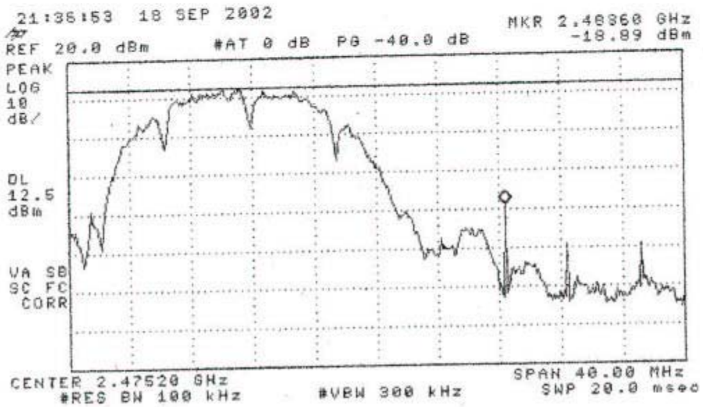
Figure 6.4(a) Band-edge behavior at low end and high end of the band.
