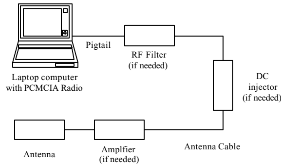
Figure 3.1 Basic block diagram of the system
