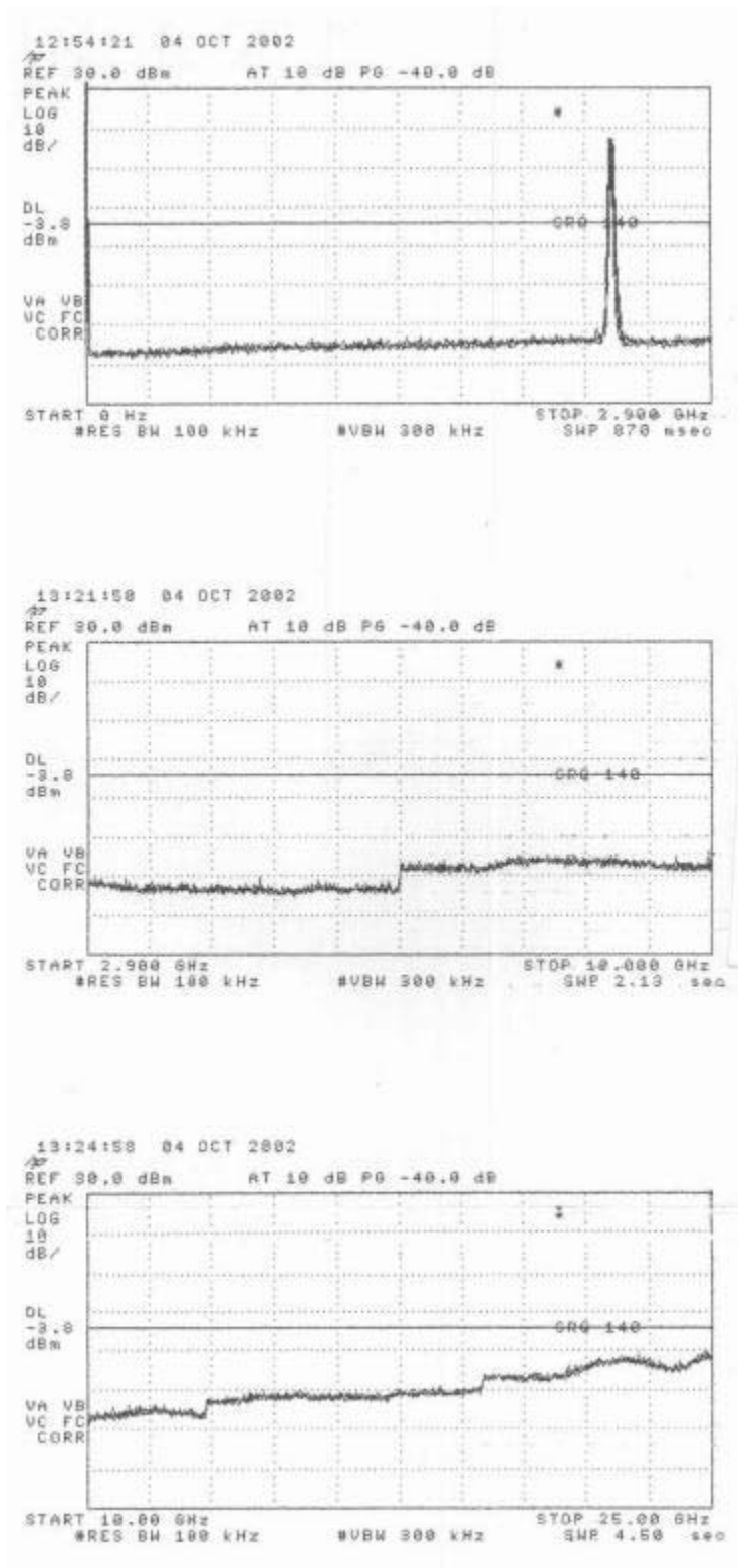
Figure 6.3(b) Antenna conducted spurious emissions; low, mid, and high channels.
