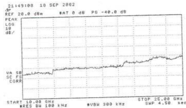
Figure 6.3(a) Antenna conducted spurious emissions; low, mid, and high channels. HA2401-AGC-250 Amplifier (250 mW)
