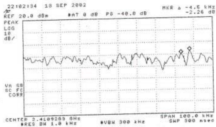
Figure 6.5(a) Spectral Density (low channel) (top) Spectrum Scan, (mid) Spectral Density, (bottom) Line Spacing. HA2401-AGC-250 Amplifier (250 mW)
