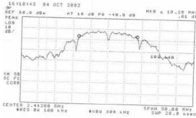
Figure 6.2(b) 6 dB-point bandwidth measurements; low, mid, and high channels. HA2401-AGC1000 Amplifier (1000 mW)
