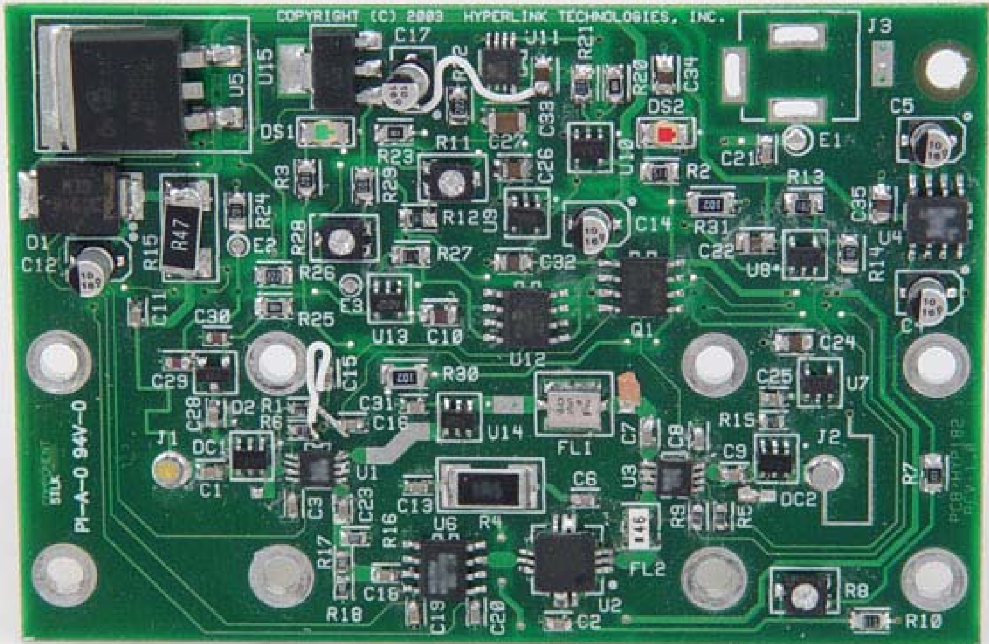
PCB (bottom)
