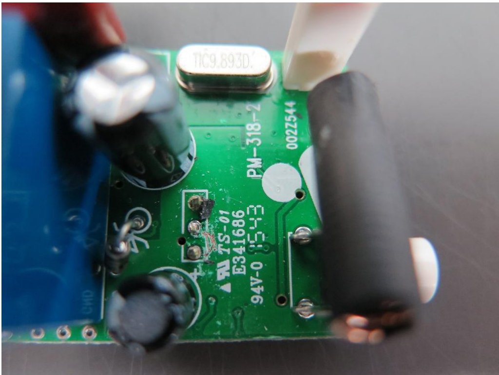
InPho4-MainBoard
