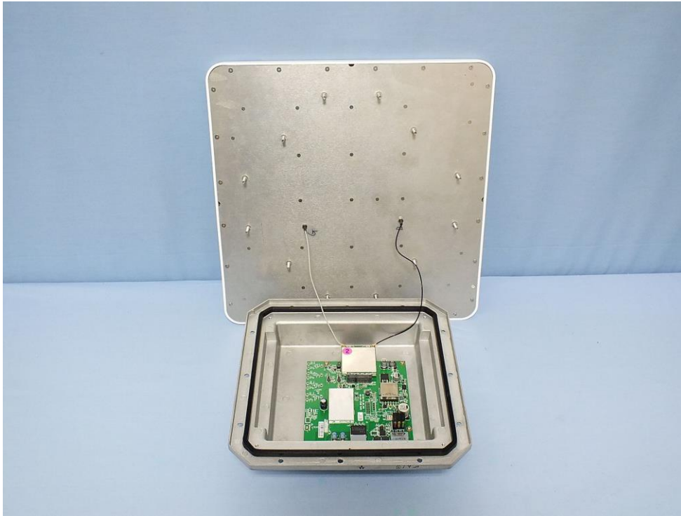
Antenna with 19.44 dBi gain
