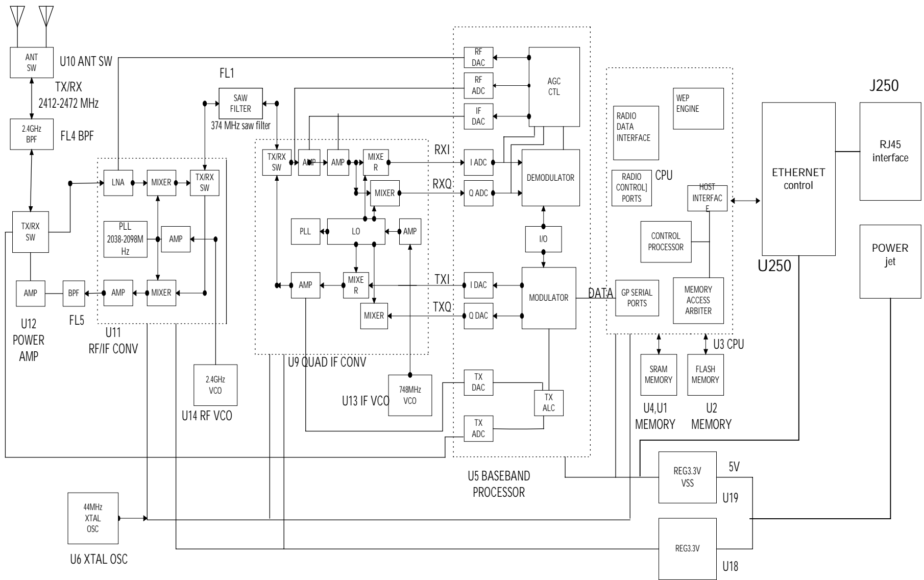
WX1560 BLOCKDIAGRAM
