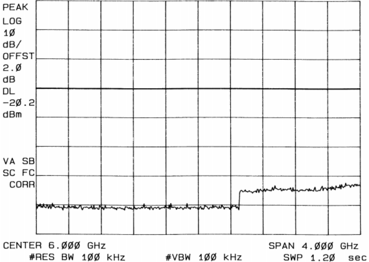
Plot 9.5: Conducted emissions 4.0 GHz – 8.0 GHz
