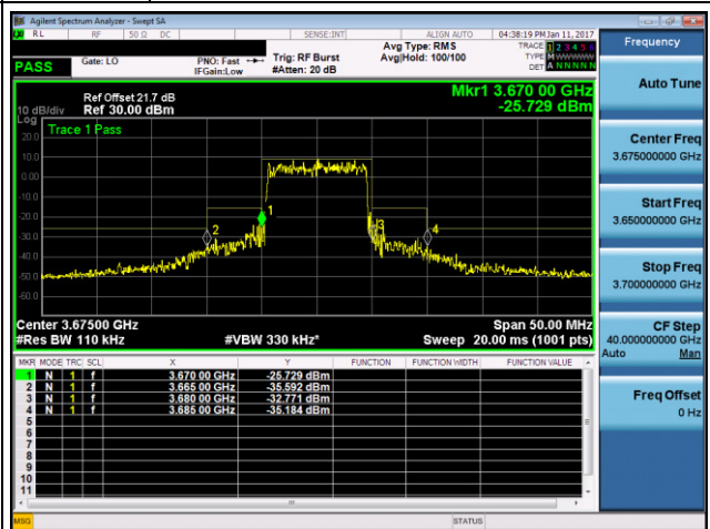
Mode CB: 10MHz , 16QAM, High channel
