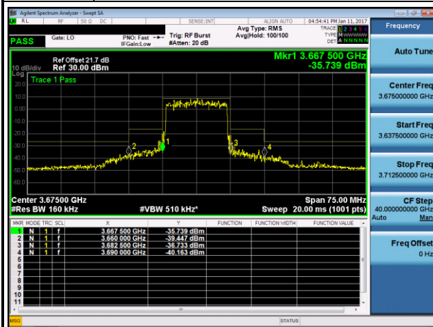
Mode CB: 15MHz , QPSK, High channel
