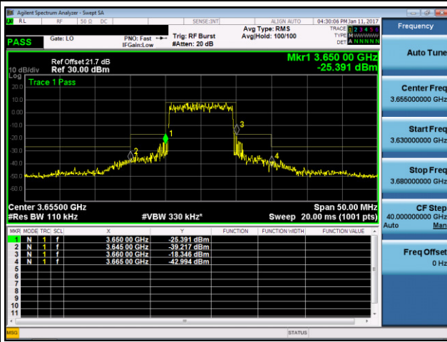
Mode CB: 10MHz , QPSK, Mid. channel
