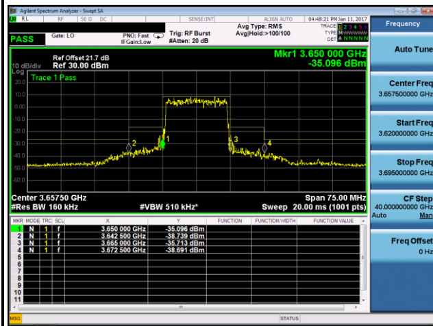
Mode CB: 15MHz , QPSK, Mid. channel
