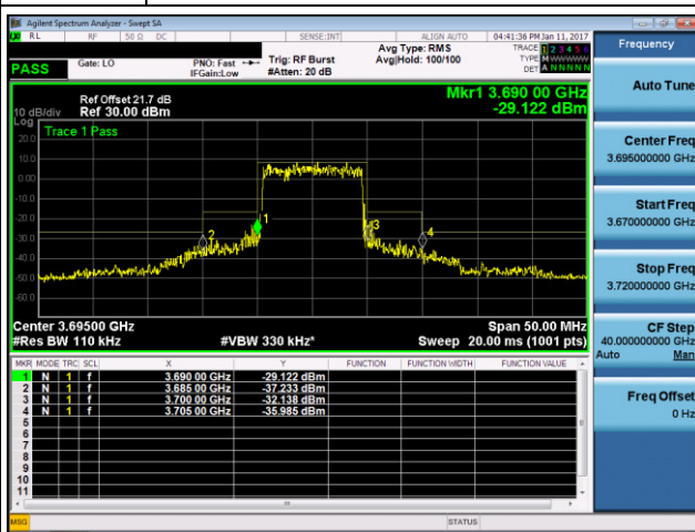
Mode CB: 10MHz , QPSK, High channel
