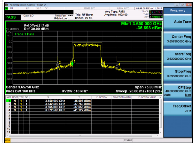
Mode CB: 15MHz , 16QAM, Mid. channel
