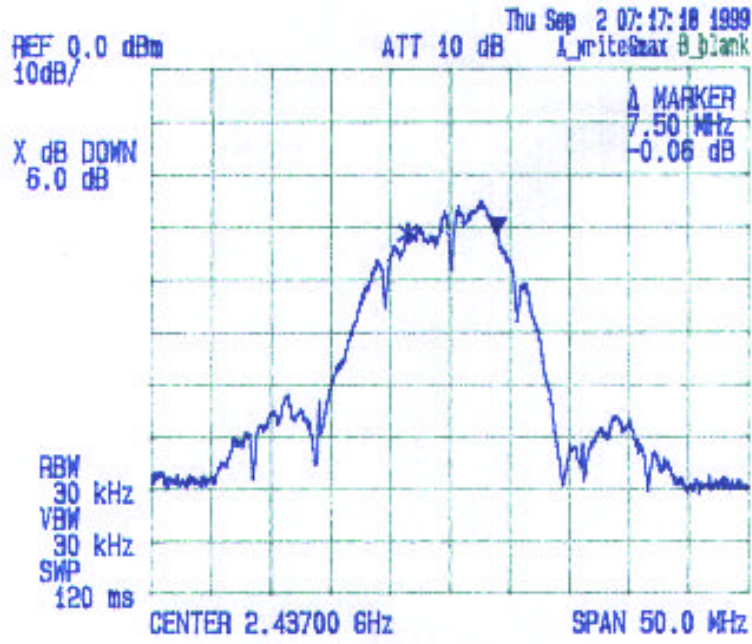
1 Mbps DBPSK
