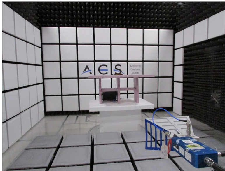
Figure 4: Radiated Emissions – Above 1GHz
