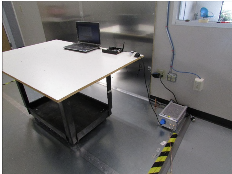
Figure 2: Powerline Conducted Side View
