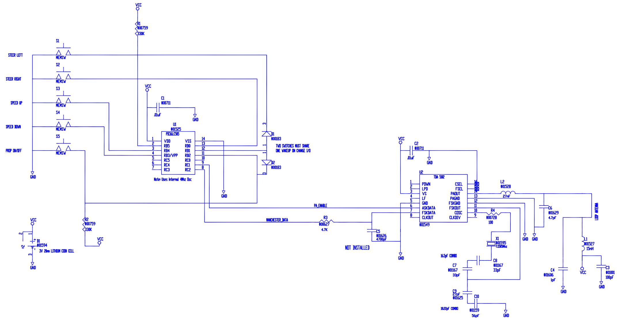
SCHEMATIC DIAGRAM, 915MHZ TRANSMITTER
