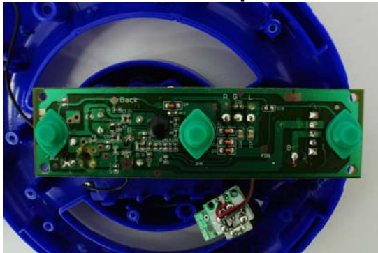
Inner Circuit Top View
