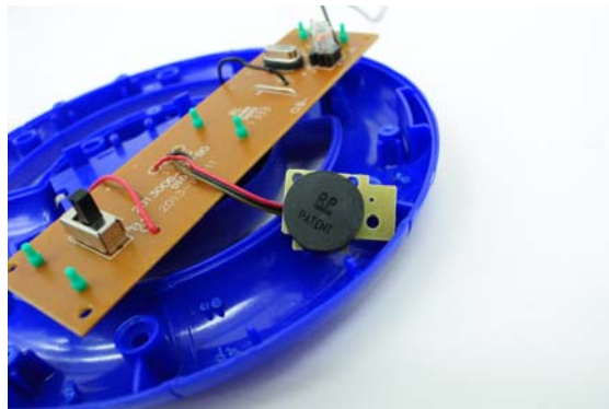
Inner Circuit Bottom View
