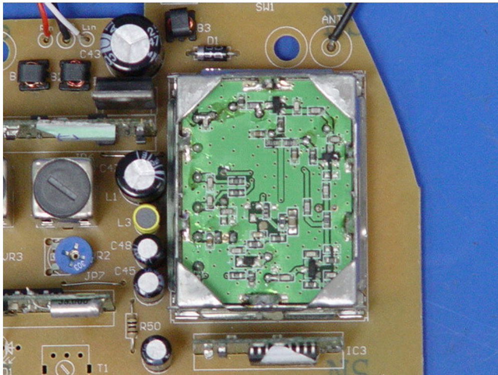
Picture of 1551 UHF module
