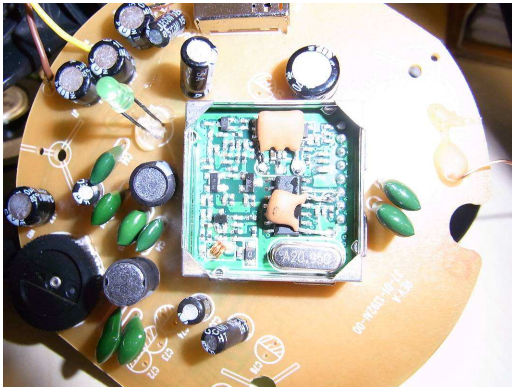
Fig. 6: Internal view
