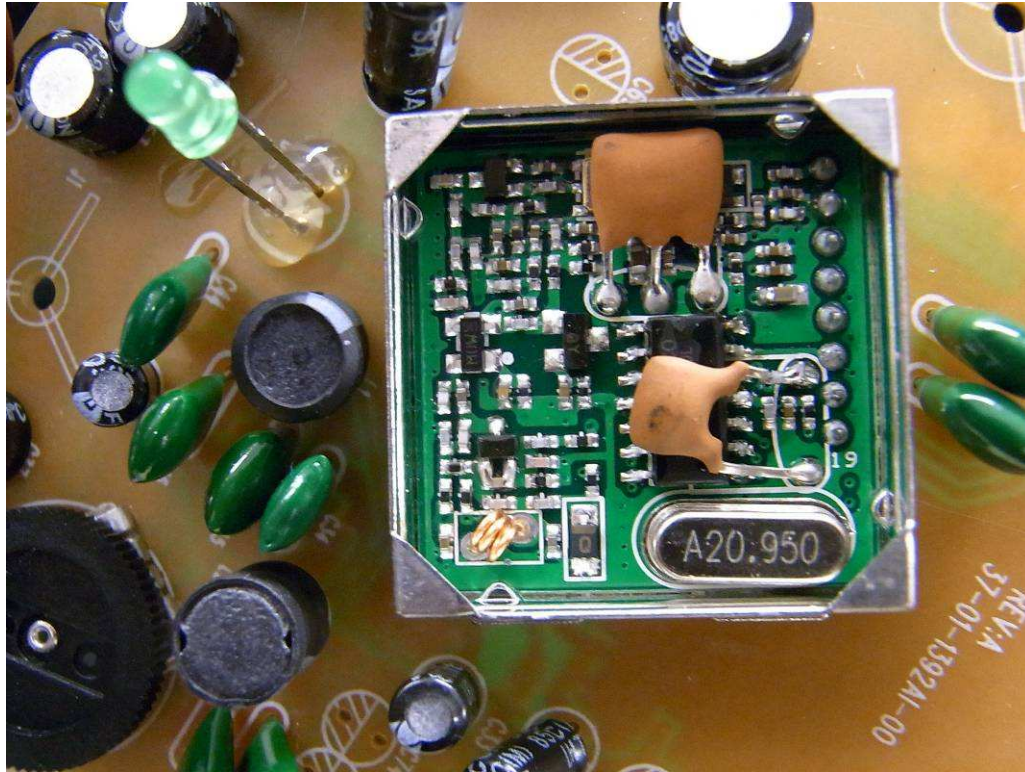
Fig. 7: Internal view
