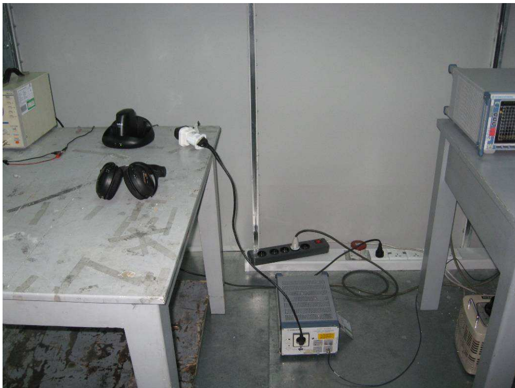
Photograph 4: Set-up for Conducted Emissions
