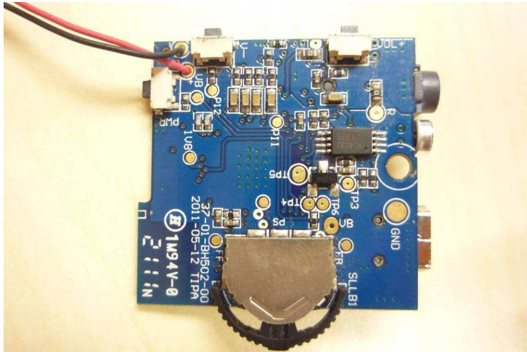
Fig. 3: Internal view
