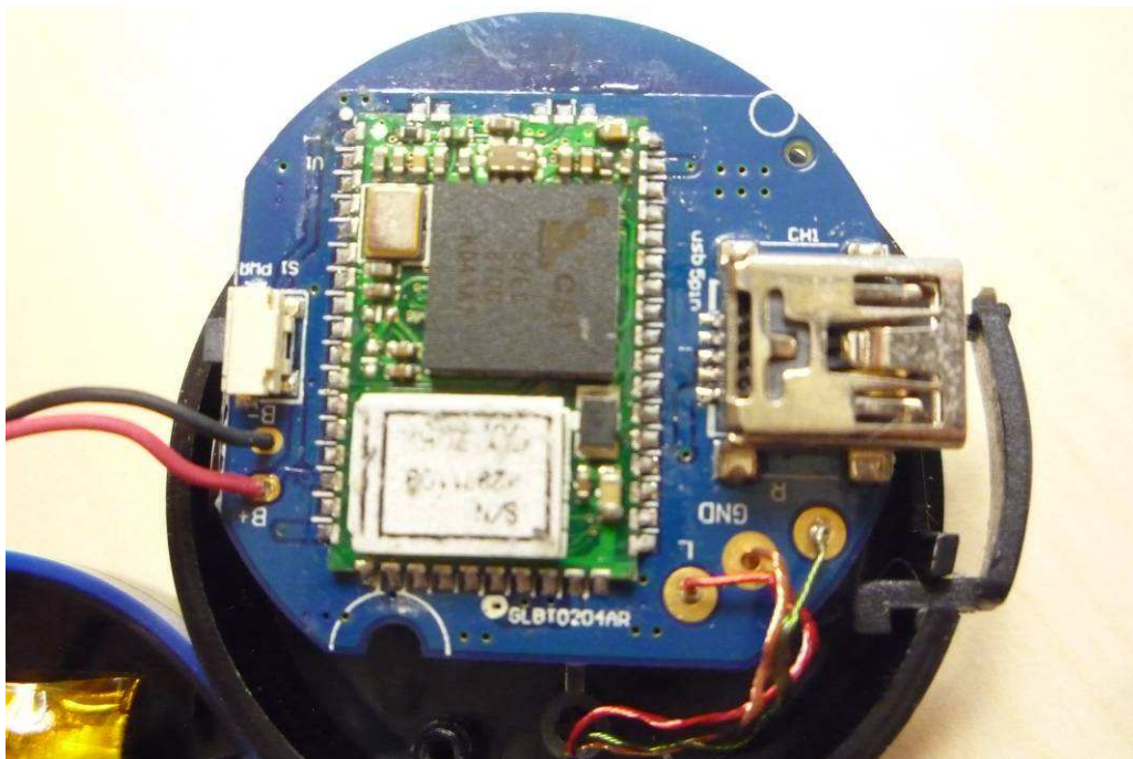
Fig. 2: Internal view
