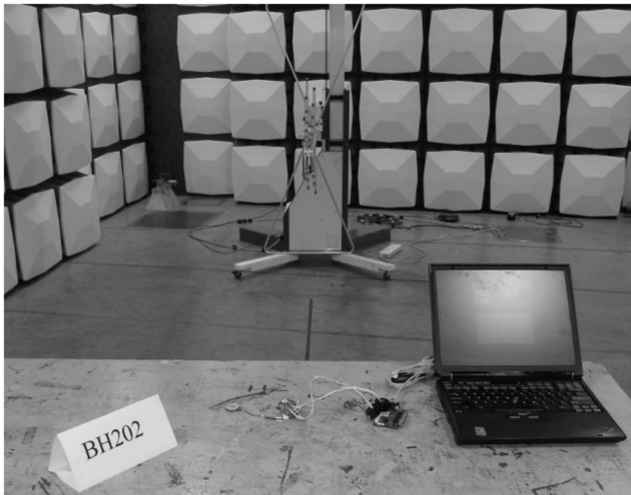
Photograph 2: Set-up for Radiation Measurement below 1GHz
