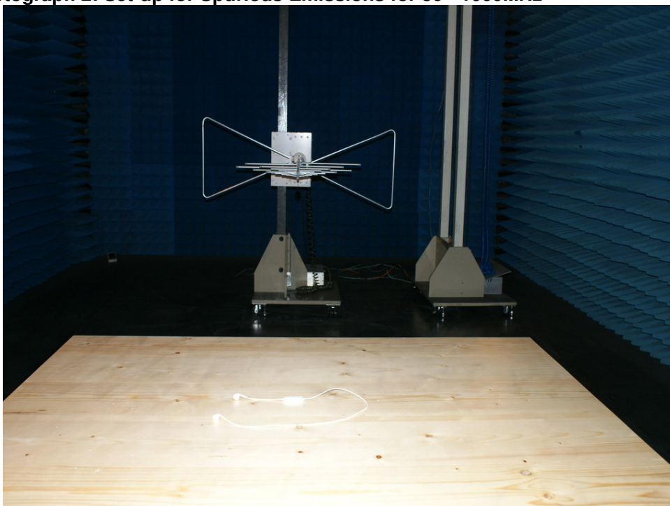
Photograph 2: Set-up for Spurious Emissions for 30 - 1000MHz
