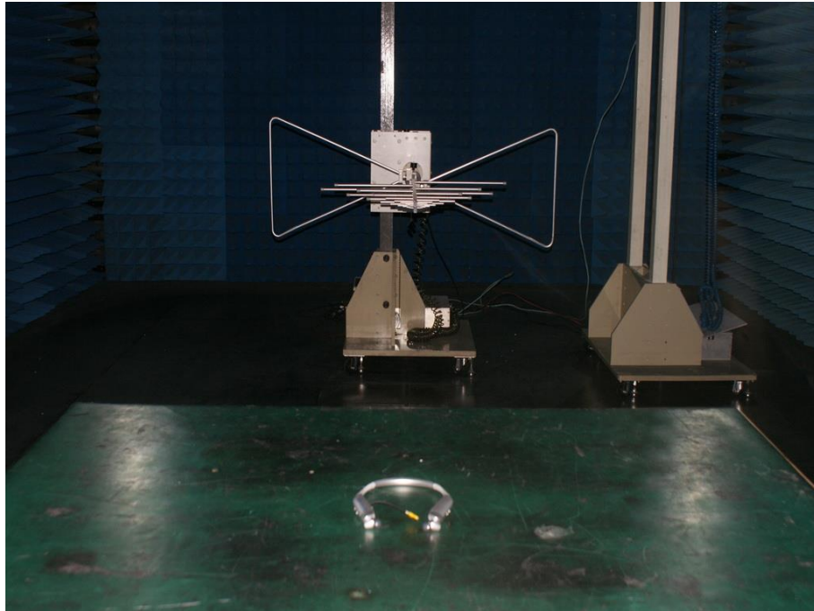
Photograph 3: Set-up for Spurious Emissions (30MHz-1GHz)
