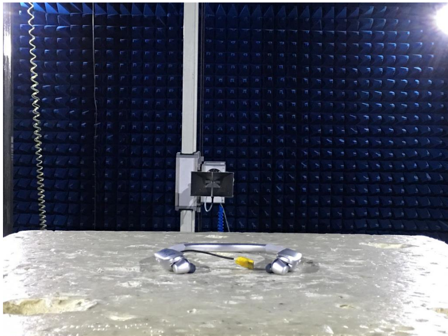
Photograph 4: Set-up for Spurious Emissions (1GHz-18GHz)
