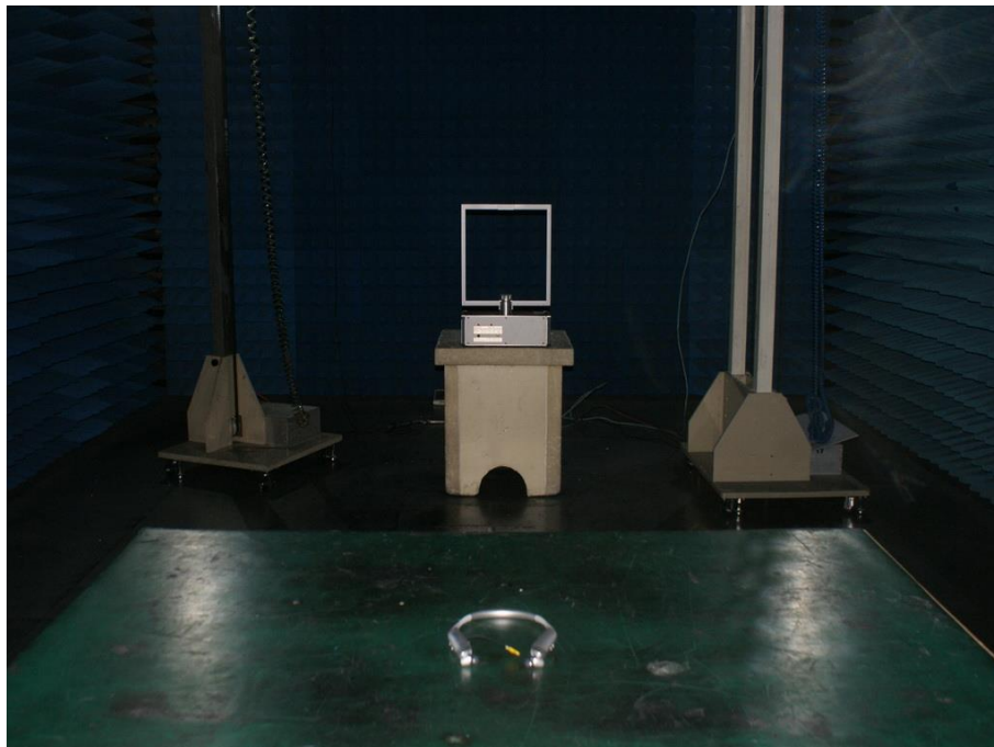
Photograph 2: Set-up for Spurious Emissions (9kHz-30MHz)
