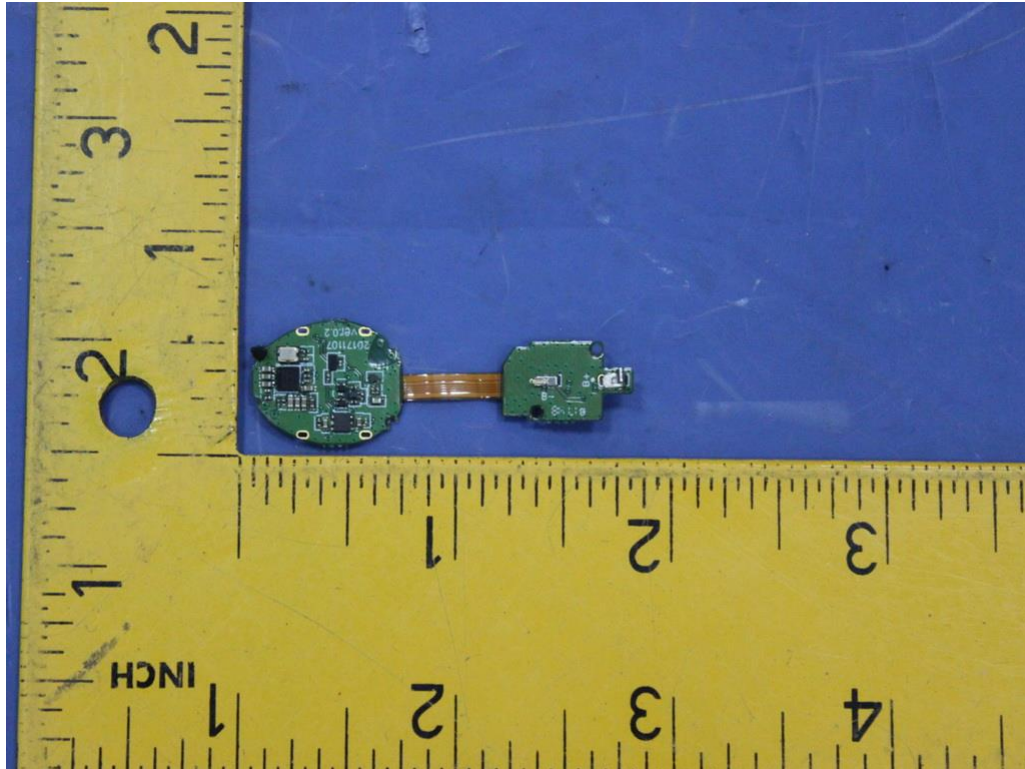
Fig. 5: Internal view
