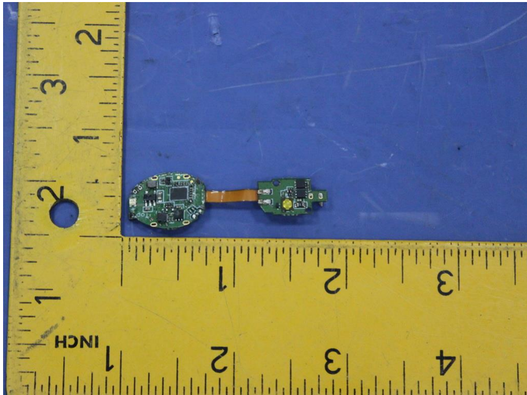
Fig. 4: Internal view
