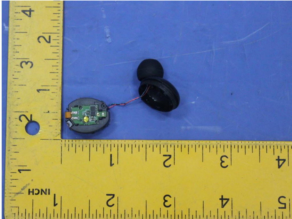
Fig. 3: Internal view
