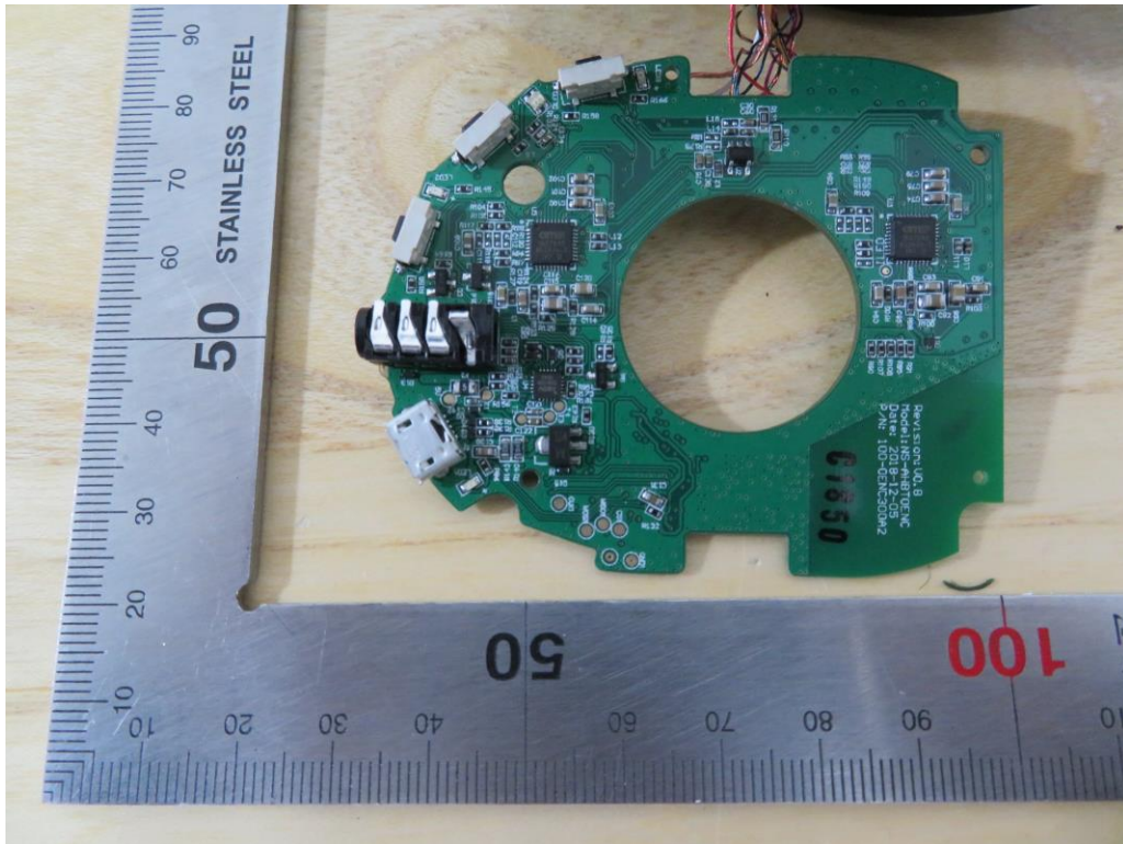
Internal View of EUT-3(left earbud)
