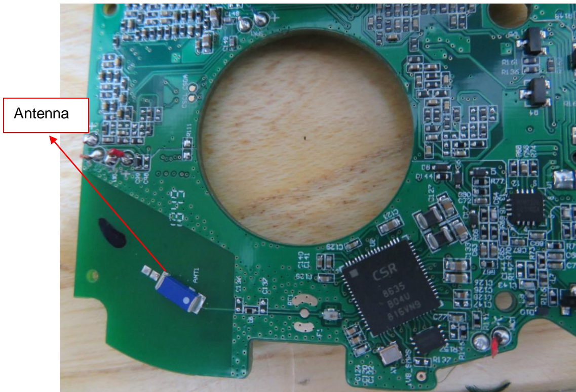
Internal View of EUT-4(left earbud)
