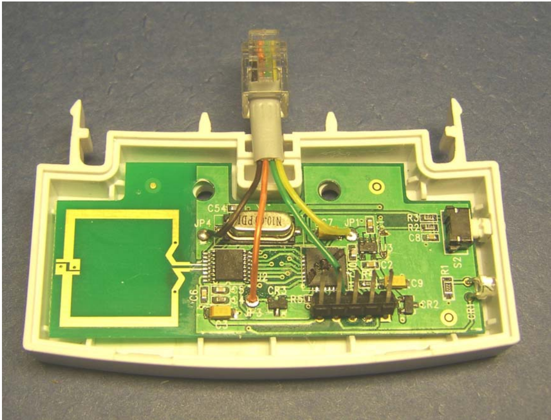
WIRELESS MODULE - INTERNAL FRONT VIEW
