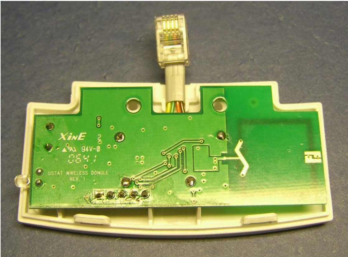
WIRELESS MODULE - INTERNAL REAR VIEW
