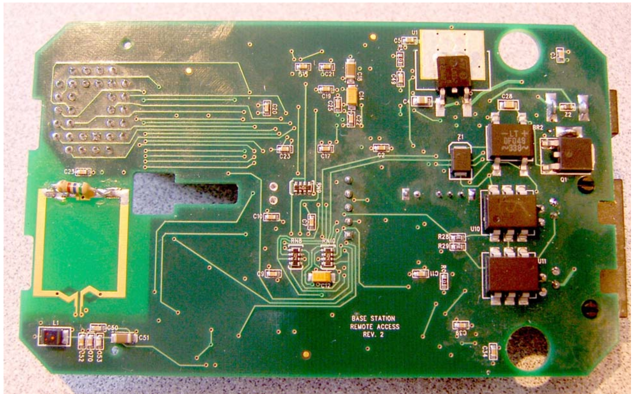
BASE STATION - INTERNAL FRONT VIEW
