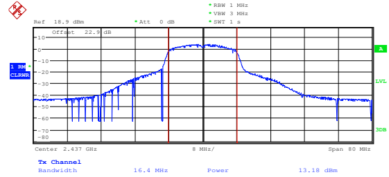
Middle channel: 2437 MHz
