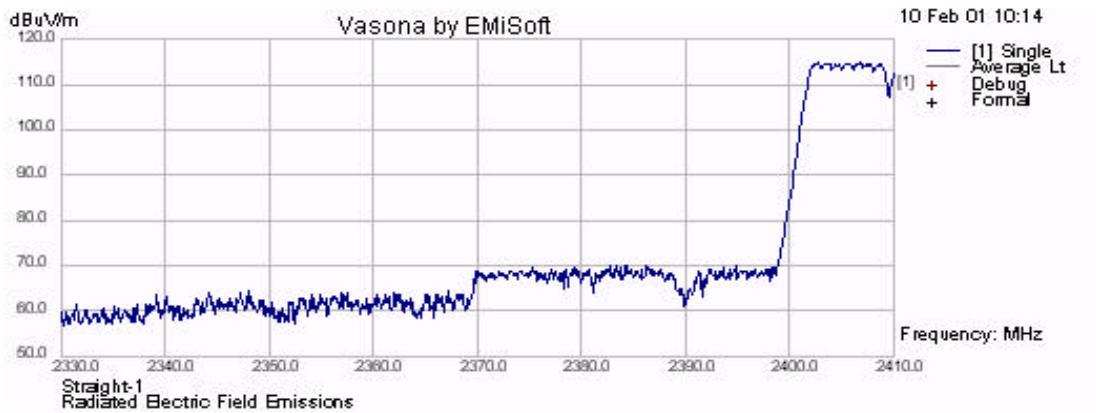
Band-edge Measurement, Low Channel, Freq. Hopping Mode
