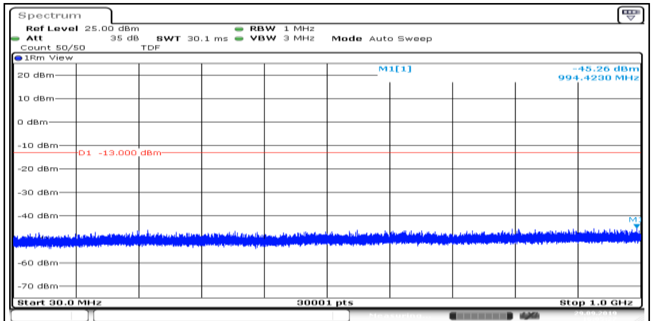
Band2_1.4MHz_QPSK_19193_1
