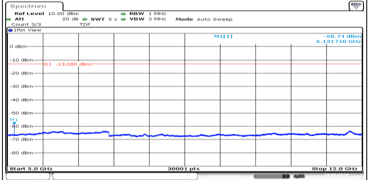
Band4_1.4MHz_QPSK_19957_6
