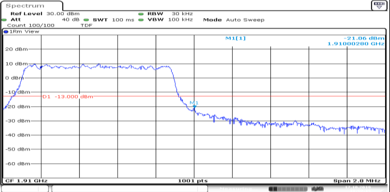
Band2_1.4MHz_QPSK_19193_6_0_Low
