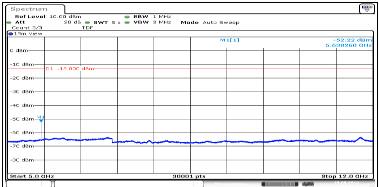
Band2_1.4MHz_16QAM_18900_1
