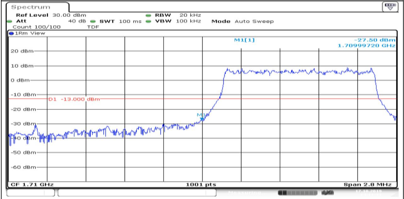
Band4_1.4MHz_16QAM_19957_6_0_Low
