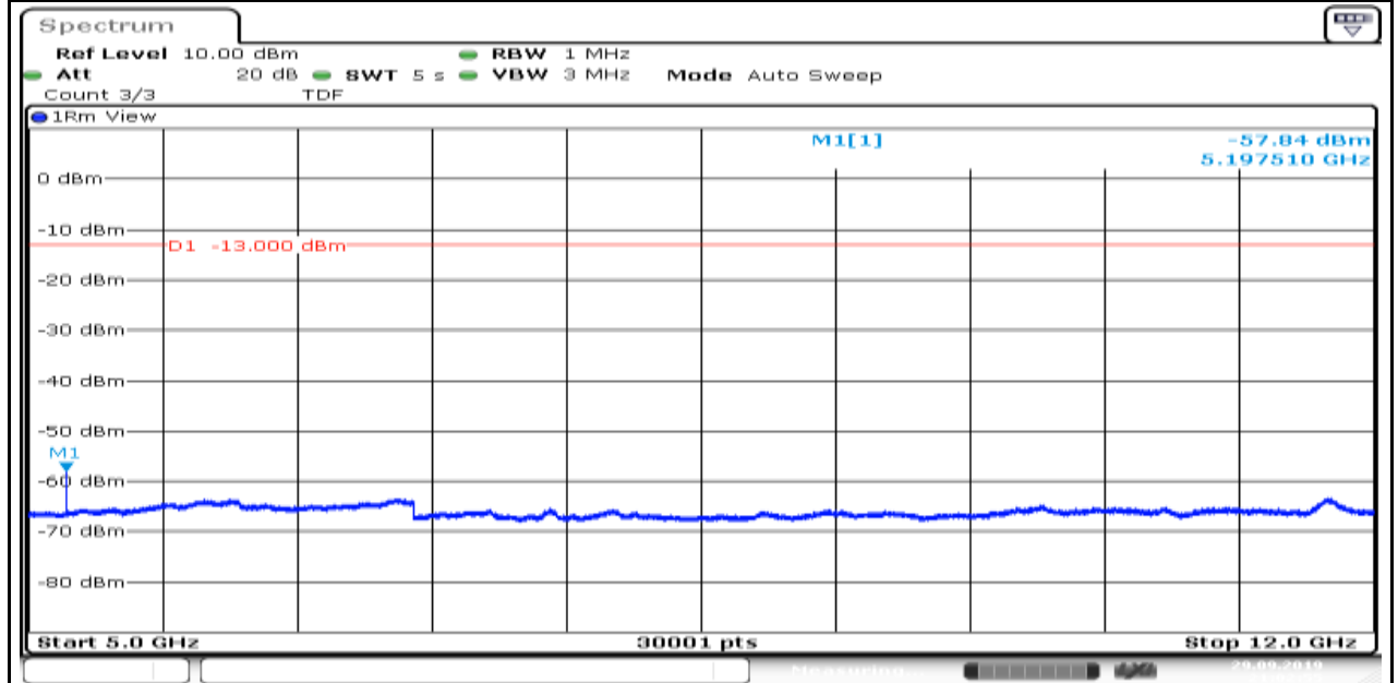
Band4_1.4MHz_16QAM_20175_6
