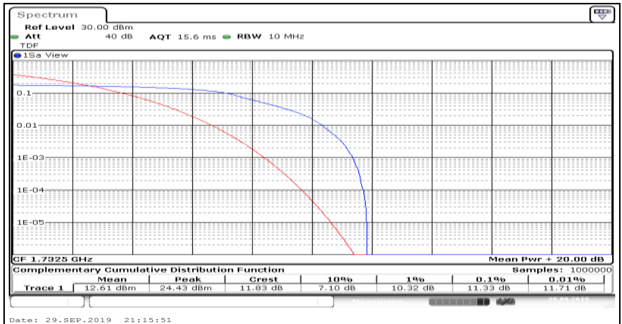
Band4_10MHz_QPSK_20175_6
