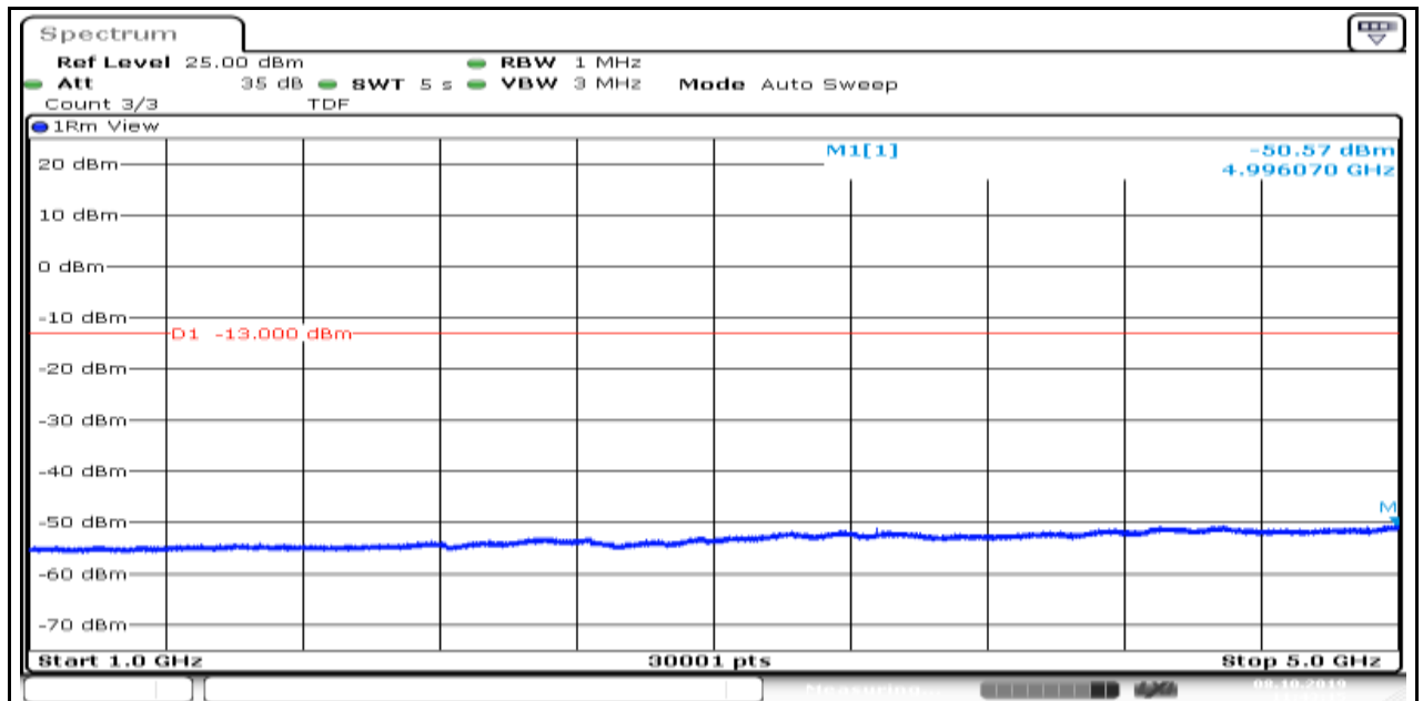
Band5_1.4MHz_QPSK_20525_1
