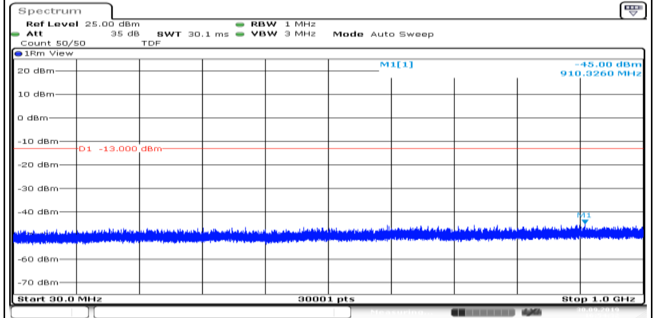
Band4_1.4MHz_QPSK_20393_1
