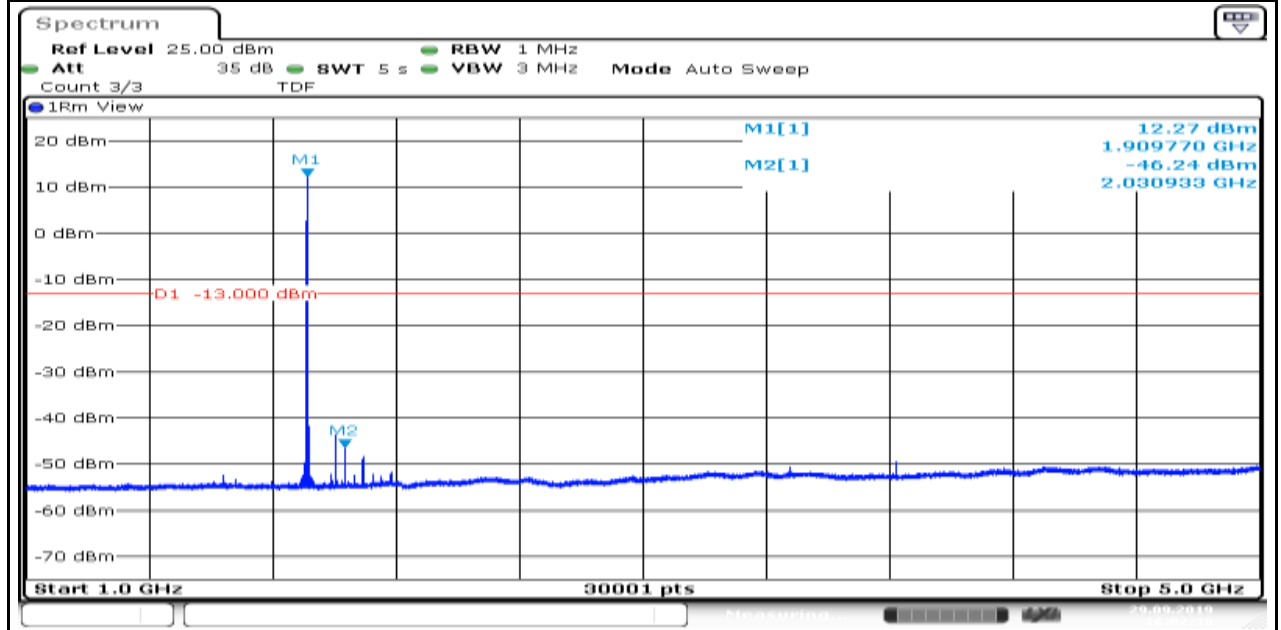
Band2_1.4MHz_QPSK_19193_1
