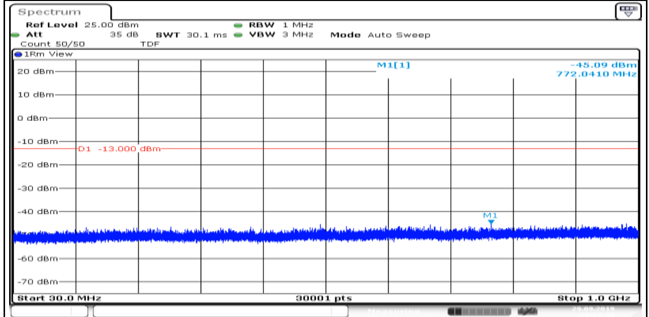
Band4_1.4MHz_16QAM_20175_1
