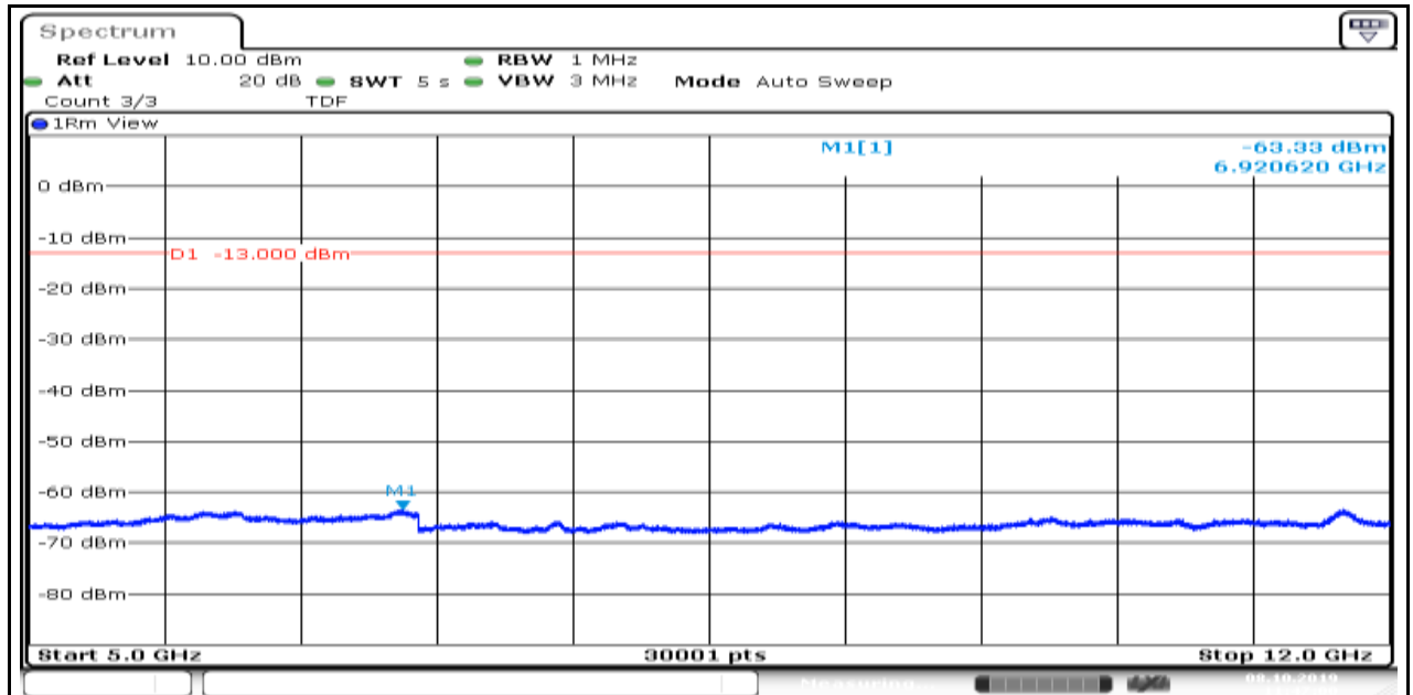
Band5_1.4MHz_QPSK_20407_1
