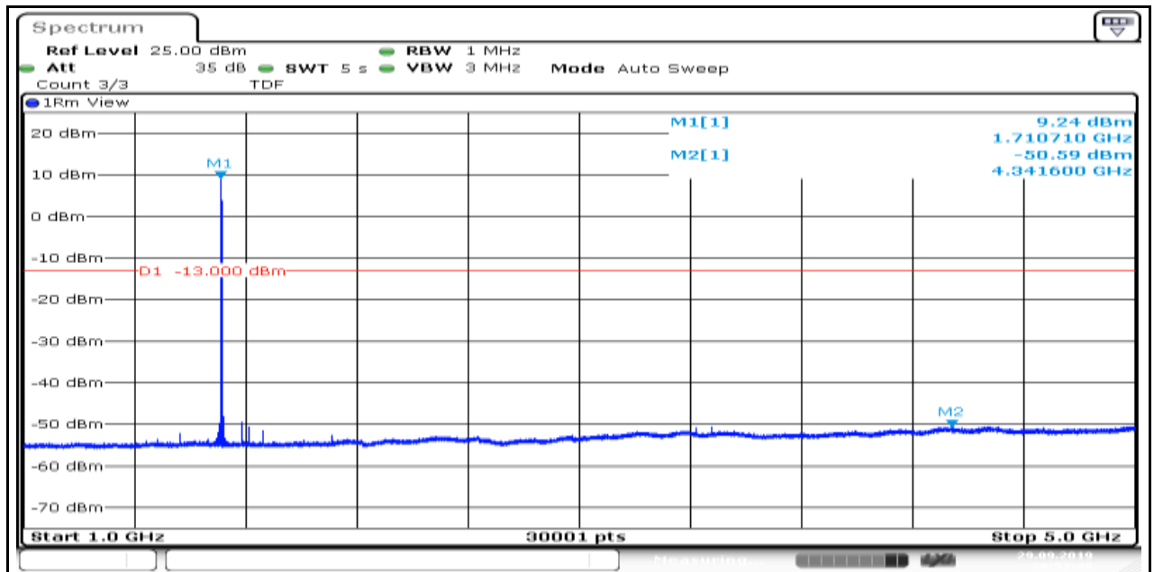
Band4_1.4MHz_QPSK_19957_6
