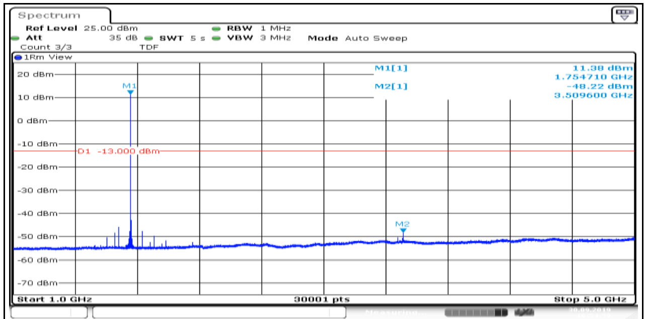
Band4_1.4MHz_QPSK_20393_1
