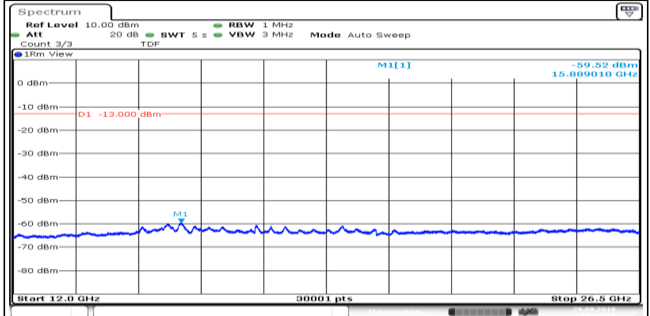
Band2_1.4MHz_16QAM_19193_6
