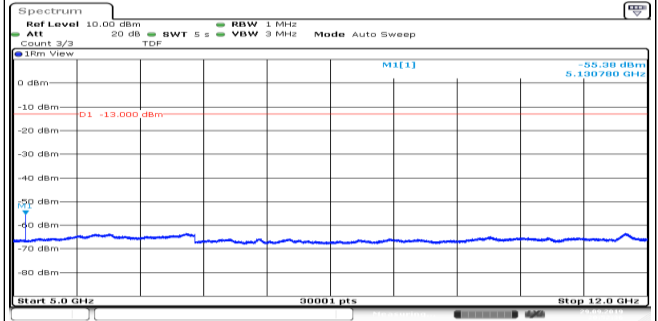
Band4_1.4MHz_16QAM_19957_1
