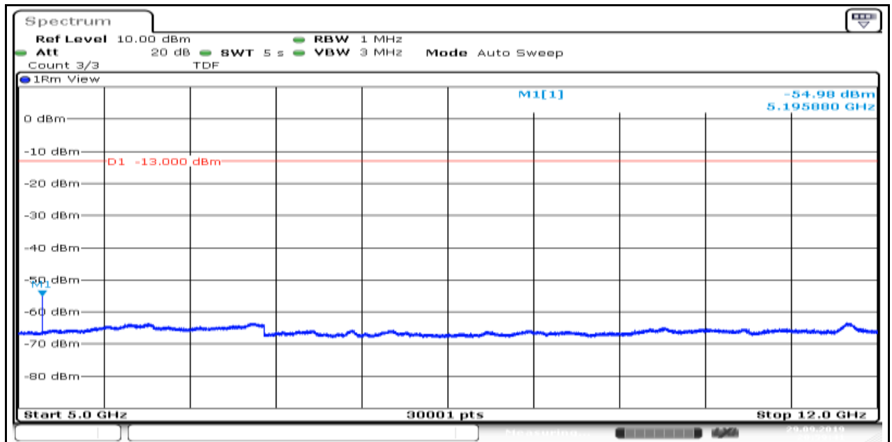
Band4_1.4MHz_16QAM_20175_1
