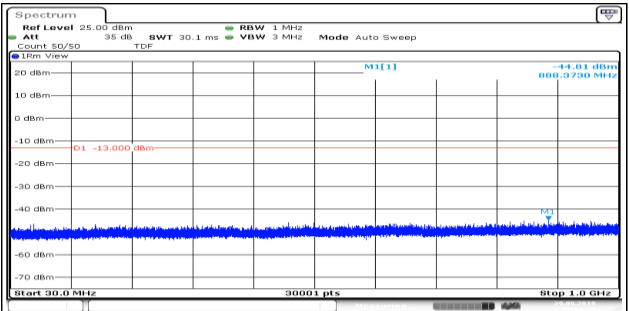
Band2_1.4MHz_16QAM_19193_1
