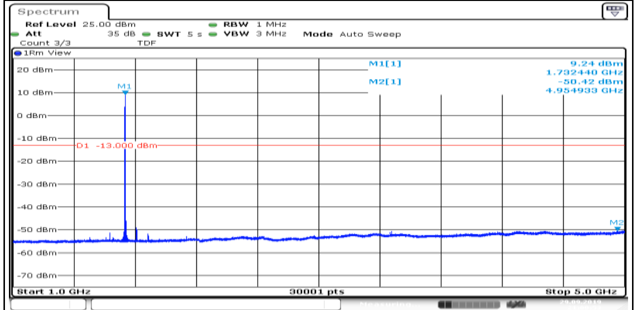
Band4_1.4MHz_QPSK_20175_6
