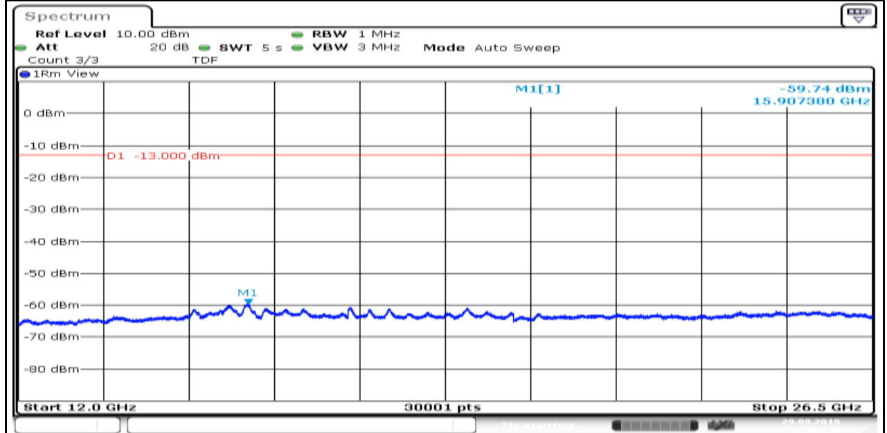
Band4_1.4MHz_16QAM_20393_5
