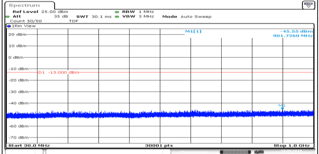
Band4_1.4MHz_16QAM_20393_5
