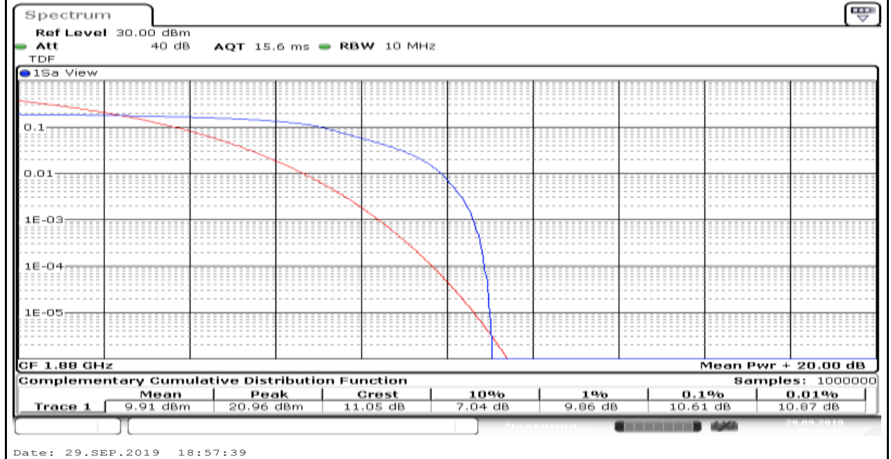
Band2_10MHz_16QAM_18900_6
