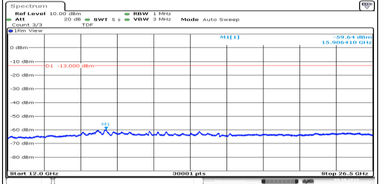
Band5_1.4MHz_QPSK_20407_1
