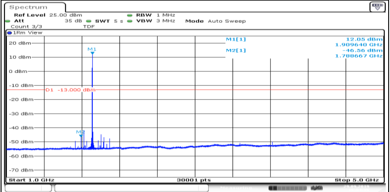
Band2_1.4MHz_16QAM_19193_1
