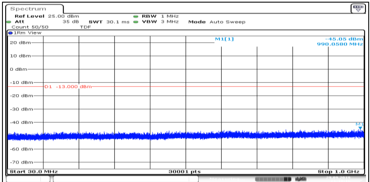
Band4_1.4MHz_16QAM_20393_5
