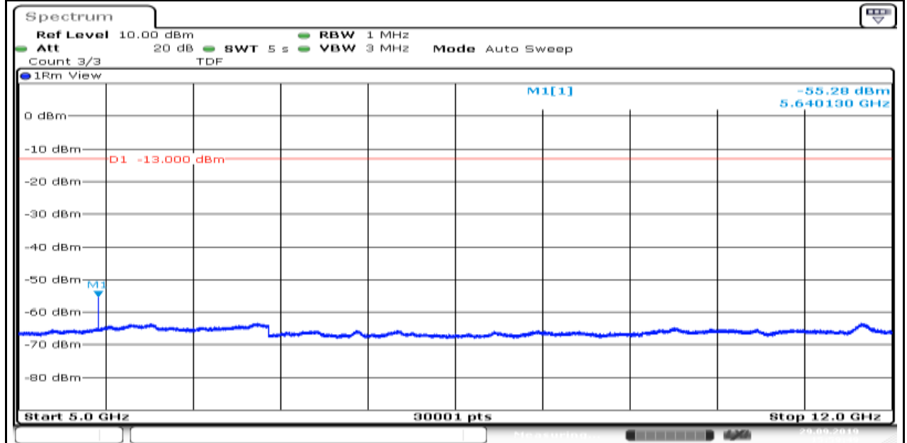
Band2_1.4MHz_QPSK_18900_6
