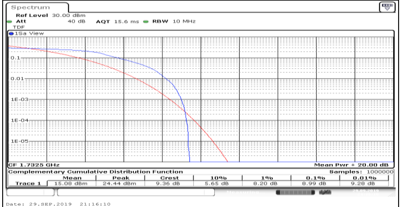
Band4_15MHz_16QAM_20175_6
