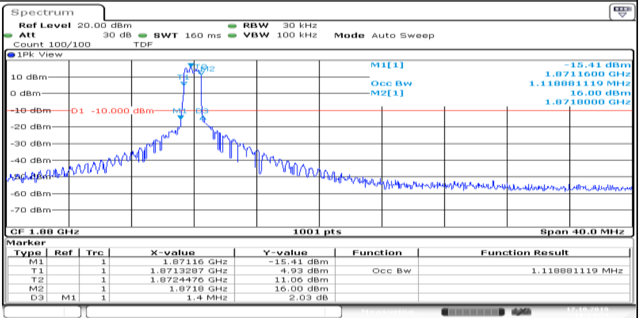
Band2_20MHz_QPSK_18900_6_0_Low
