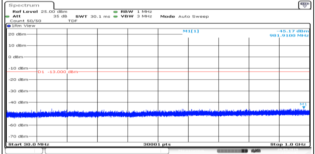
Band4_1.4MHz_QPSK_20393_5
