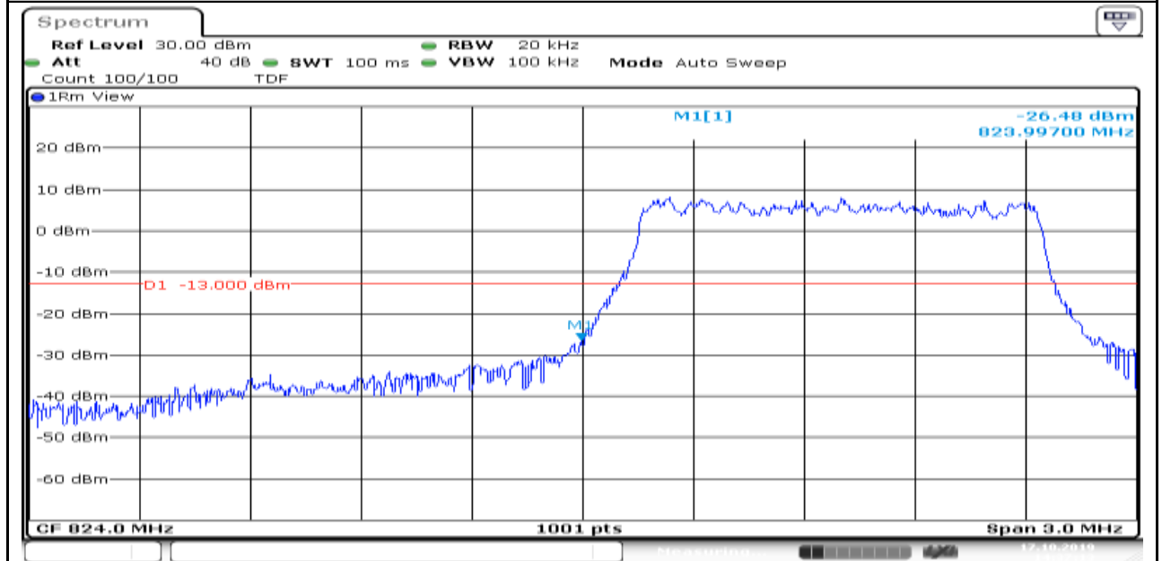
Band5_1.4MHz_16QAM_20407_6_0_Low
