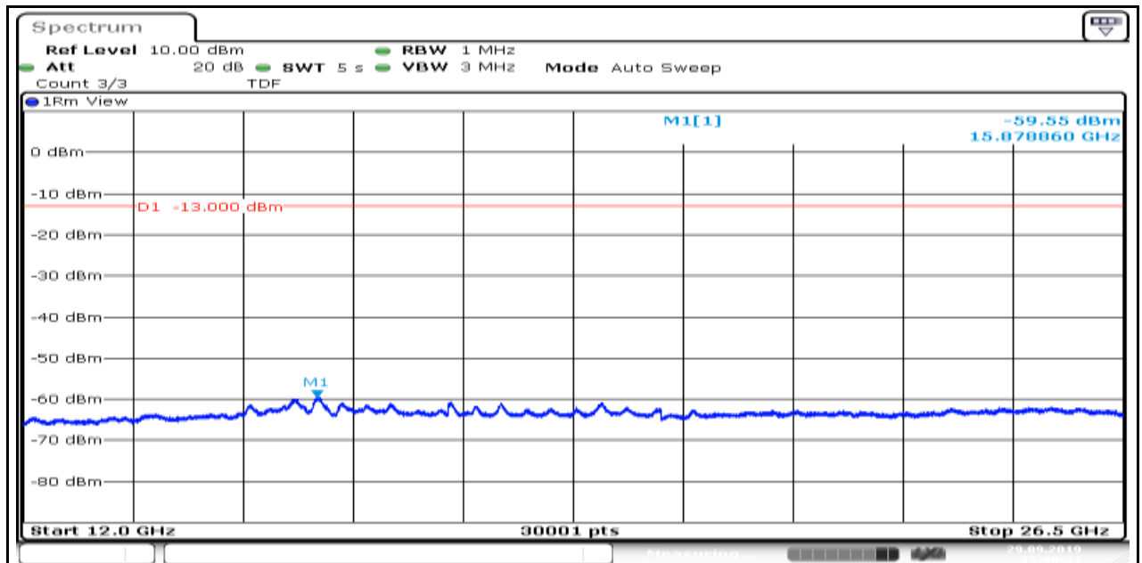
Band2_1.4MHz_QPSK_18607_6
