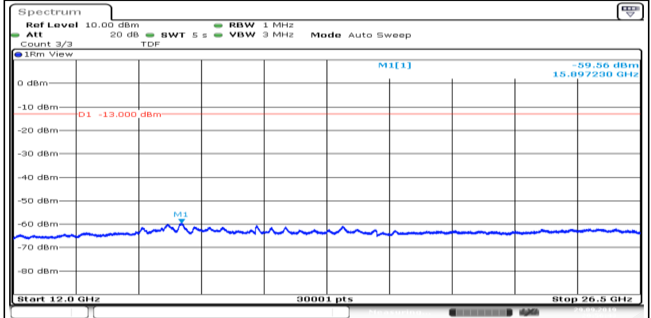
Band4_1.4MHz_16QAM_19957_6
