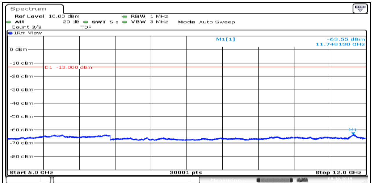
Band5_1.4MHz_QPSK_20407_6
