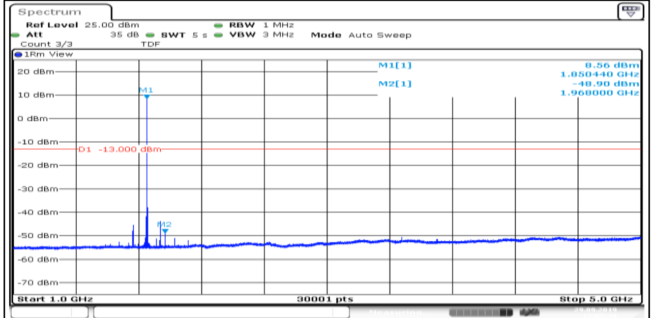
Band2_1.4MHz_16QAM_18607_6
