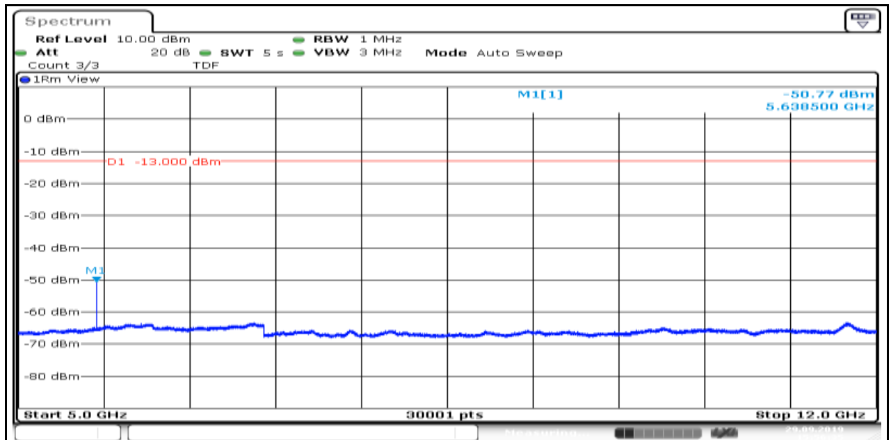
Band2_1.4MHz_QPSK_18900_1
