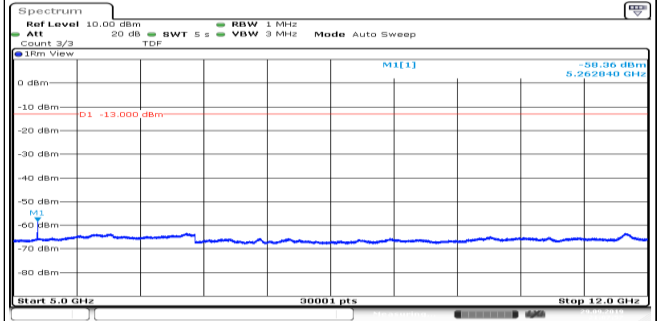
Band4_1.4MHz_QPSK_20393_6
