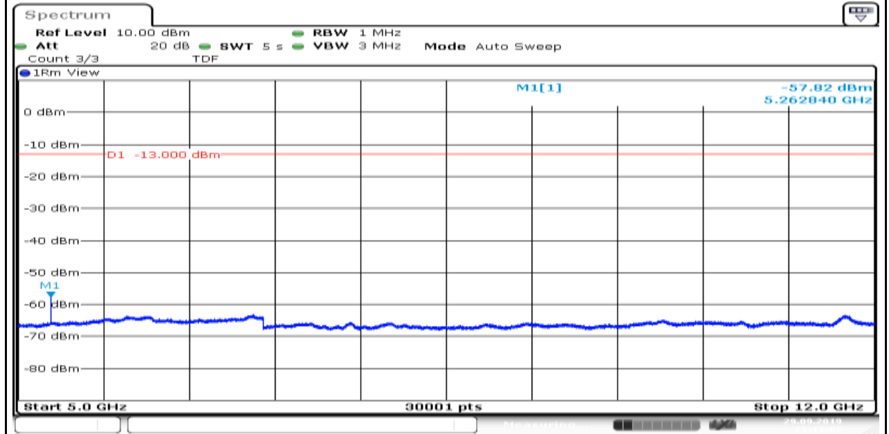
Band4_1.4MHz_16QAM_20393_6
