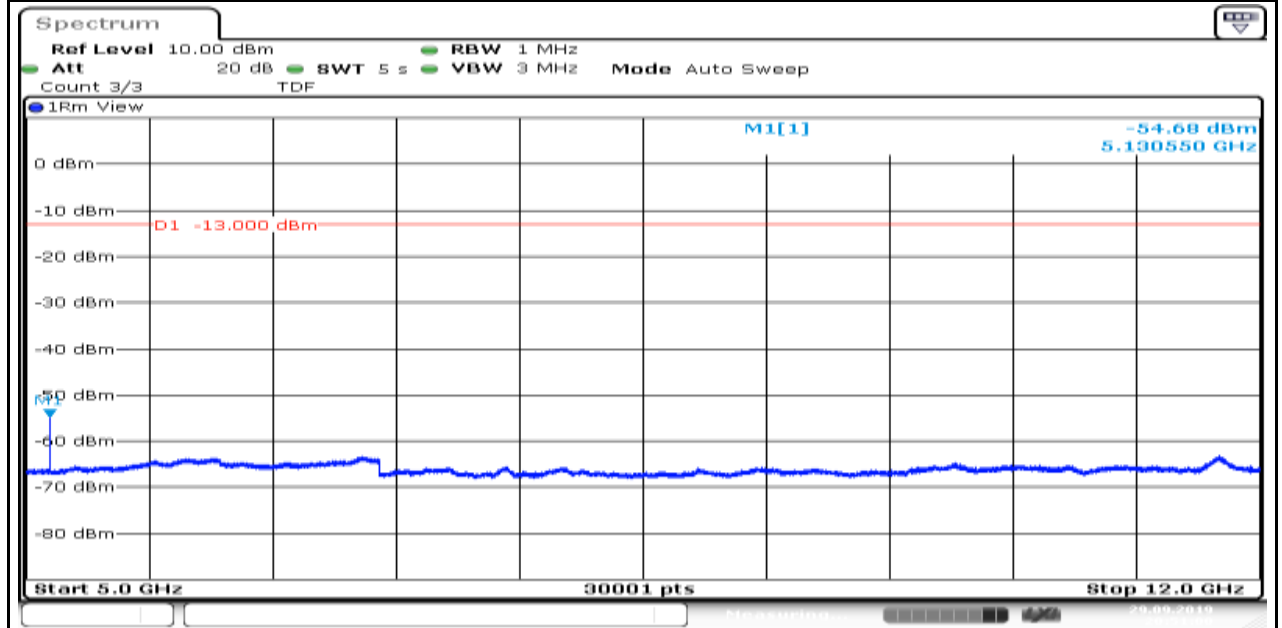
Band4_1.4MHz_QPSK_19957_1
