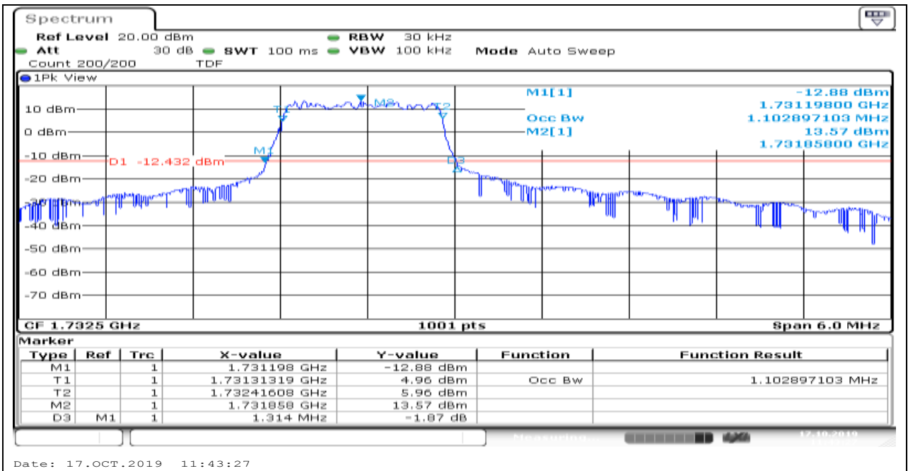
Band4_15MHz_16QAM_20175_6_0_Low
