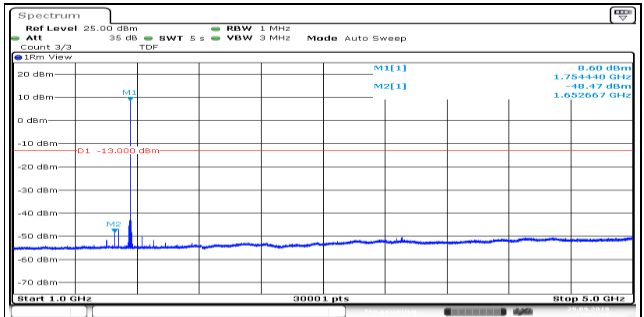
Band4_1.4MHz_16QAM_20393_5
