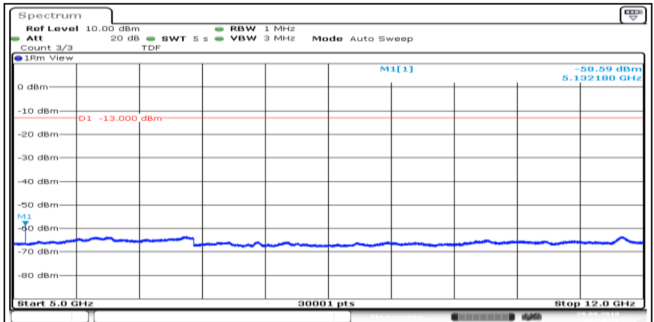
Band4_1.4MHz_16QAM_19957_6
