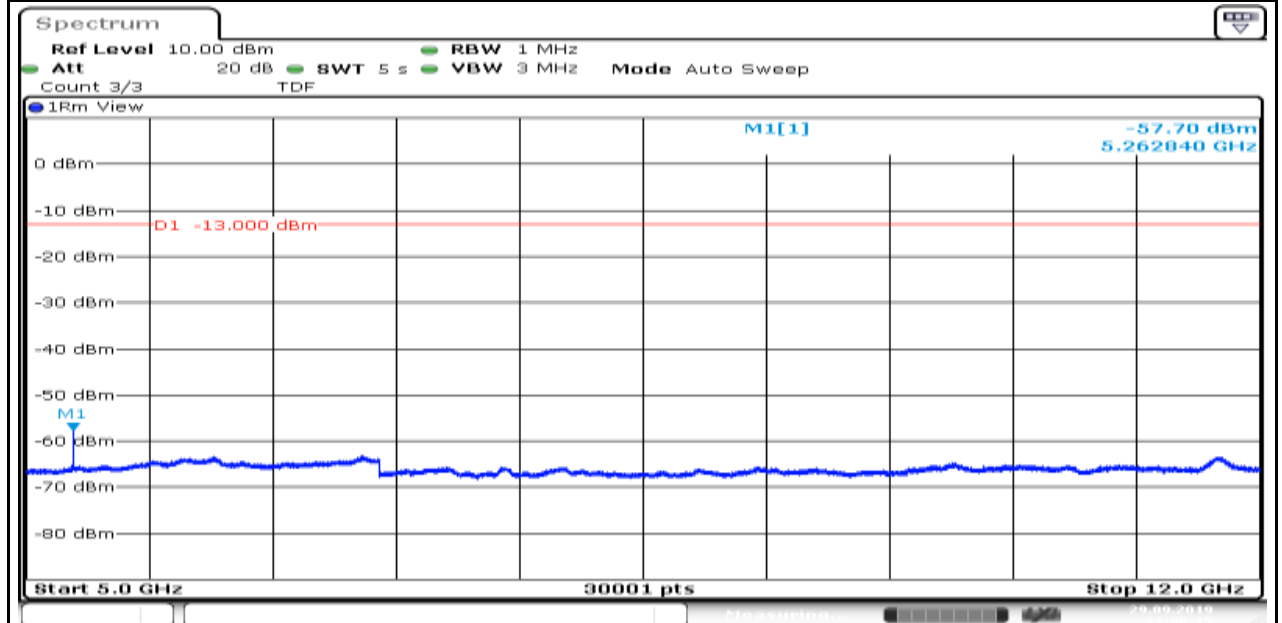
Band4_1.4MHz_16QAM_20393_5
