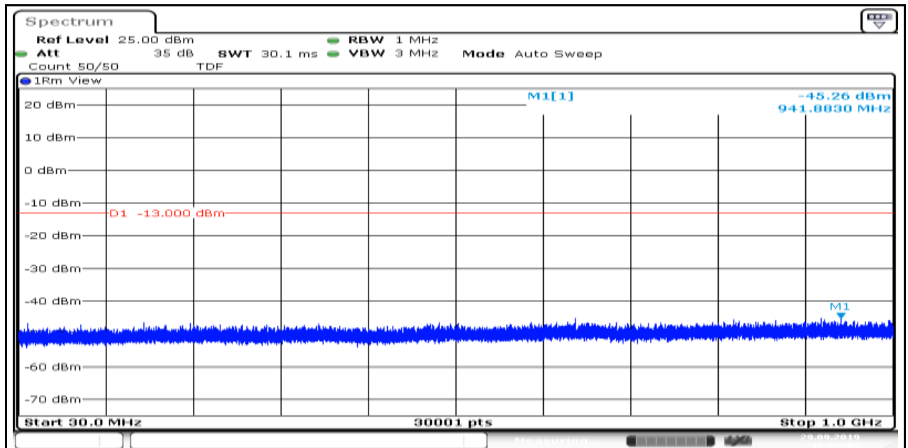
Band2_1.4MHz_16QAM_19193_6
