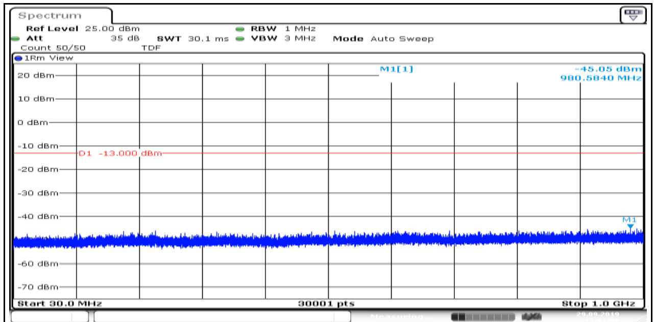
Band2_1.4MHz_16QAM_18607_1
