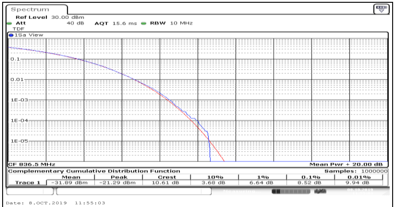
Band5_1.4MHz_QPSK_20525_6
