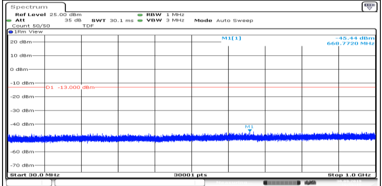
Band4_1.4MHz_16QAM_20393_1
