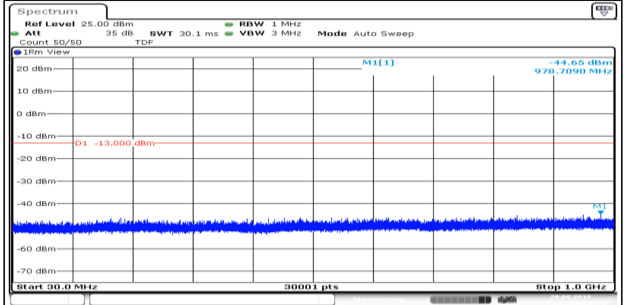
Band2_1.4MHz_QPSK_18900_1
