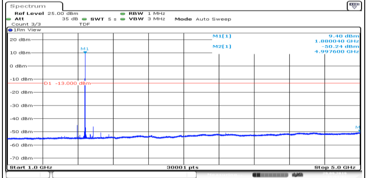
Band2_1.4MHz_16QAM_18900_6
