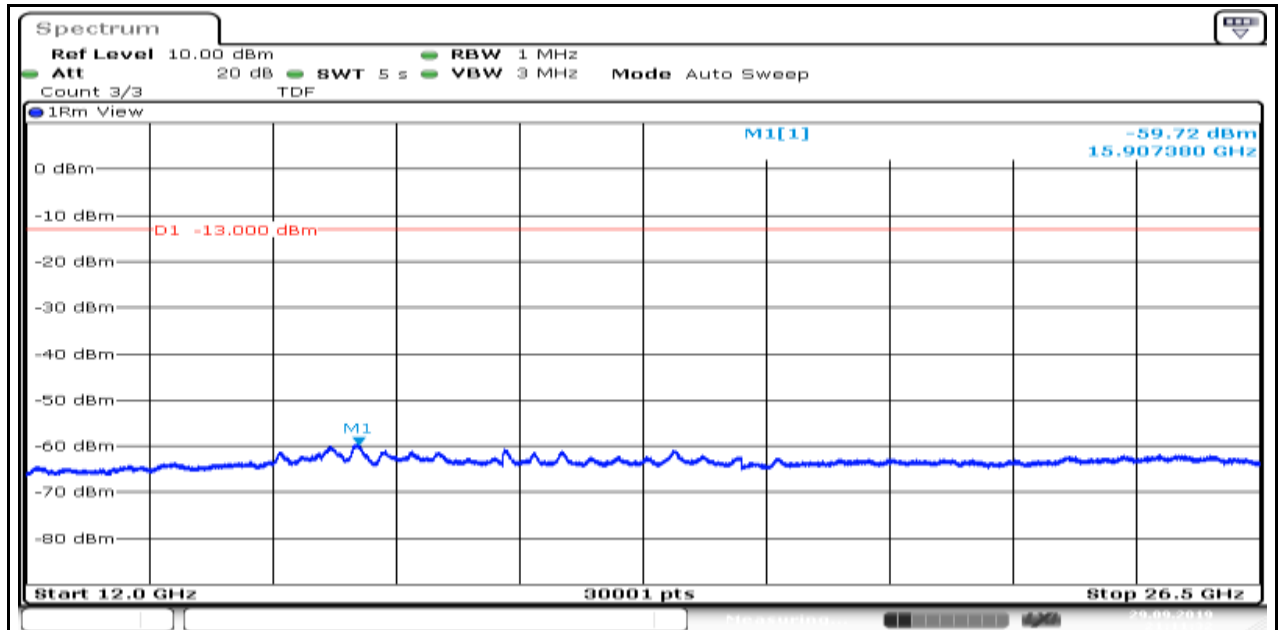
Band4_1.4MHz_16QAM_20393_6
