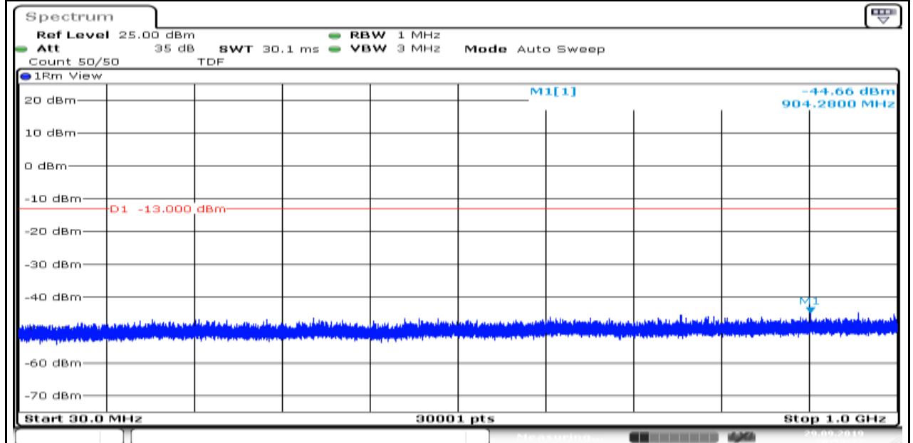
Band4_1.4MHz_QPSK_19957_6
