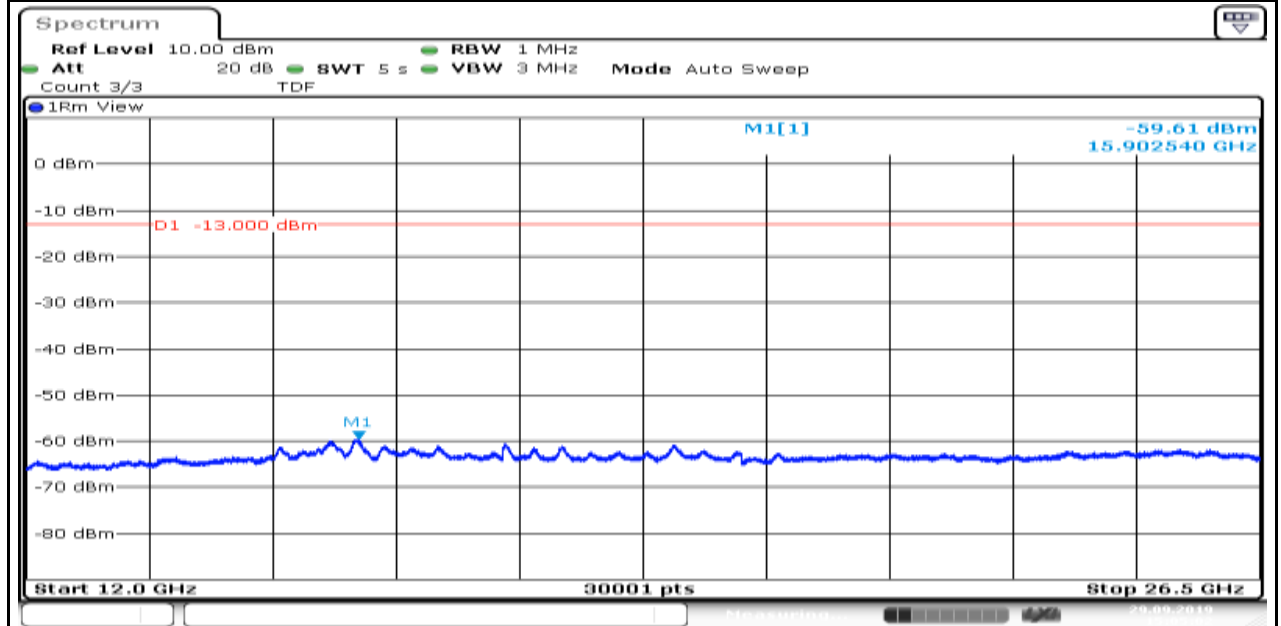
Band2_1.4MHz_QPSK_18607_6
