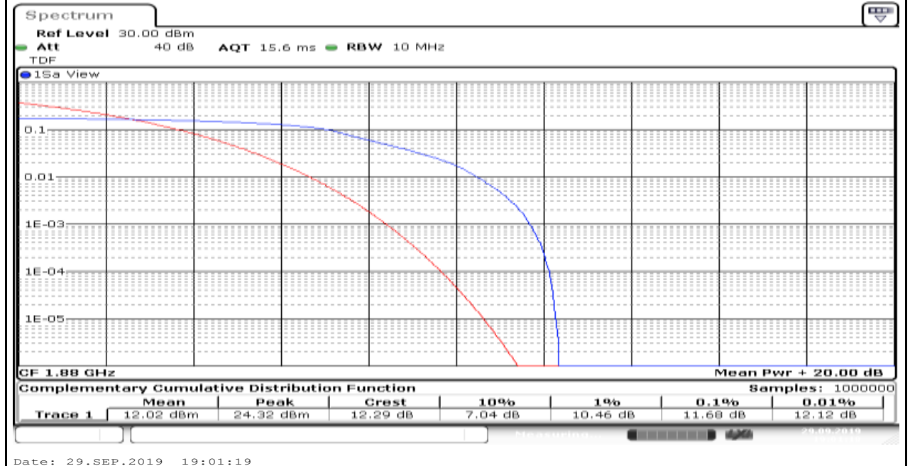
Band2_20MHz_16QAM_18900_6
