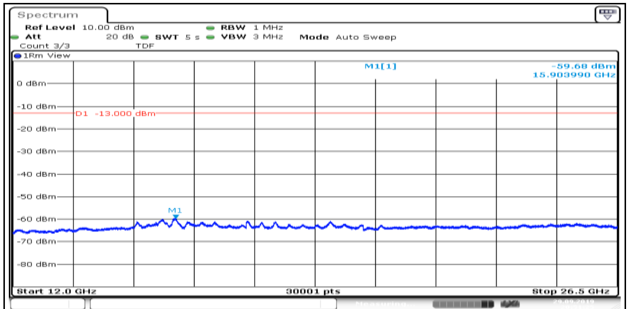
Band4_1.4MHz_QPSK_19957_6
