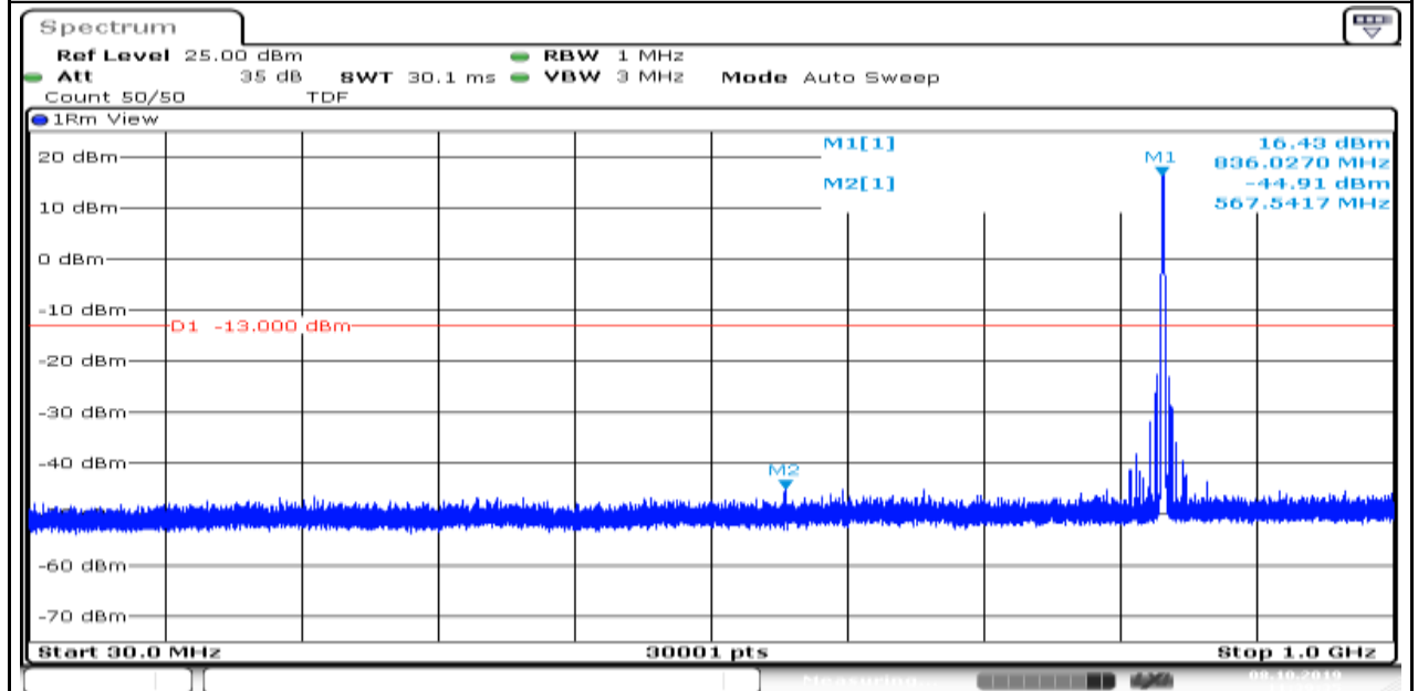
Band5_1.4MHz_QPSK_20525_1
