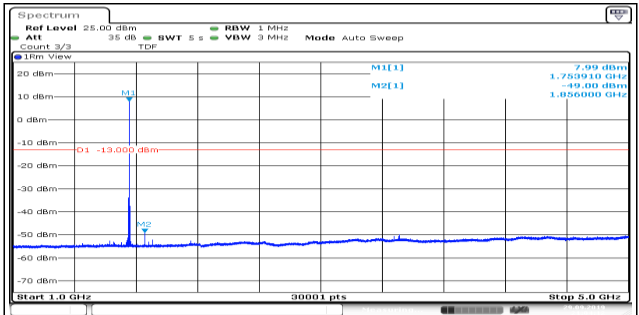
Band4_1.4MHz_QPSK_20393_5
