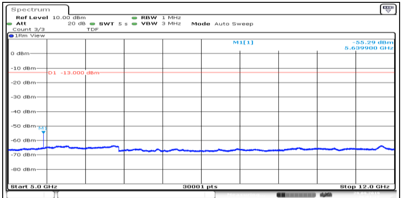
Band2_1.4MHz_16QAM_18900_6
