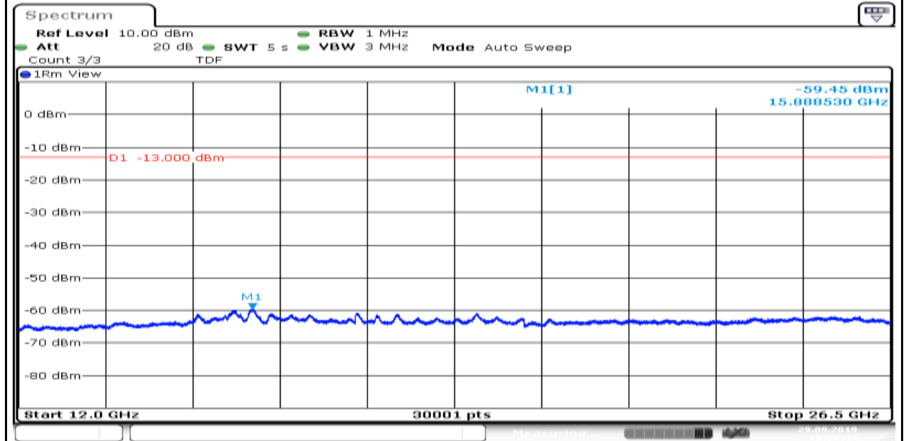
Band2_1.4MHz_QPSK_19193_6
