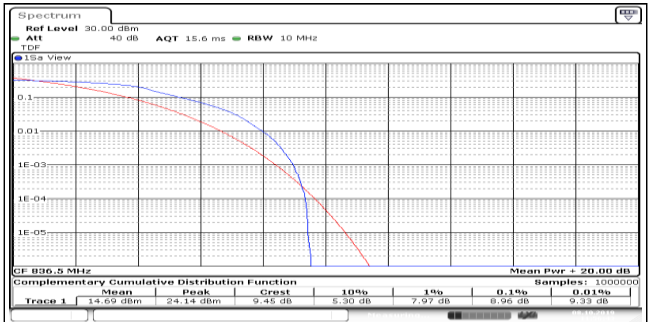
Band5_10MHz_16QAM_20525_6
