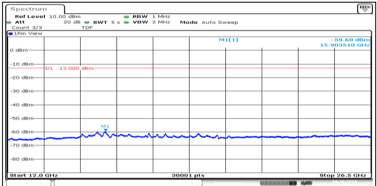
Band5_1.4MHz_QPSK_20525_1
