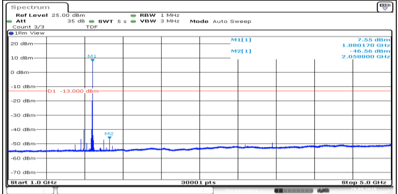
Band2_1.4MHz_QPSK_18900_1
