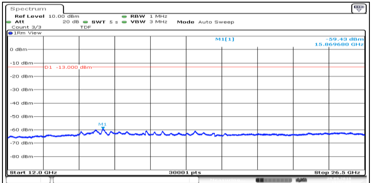
Band2_1.4MHz_QPSK_18900_1
