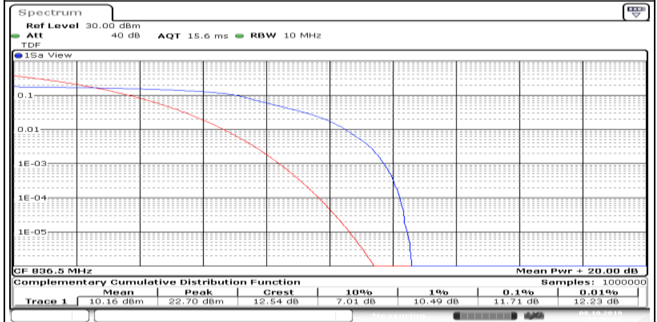
Band5_10MHz_16QAM_20525_6
