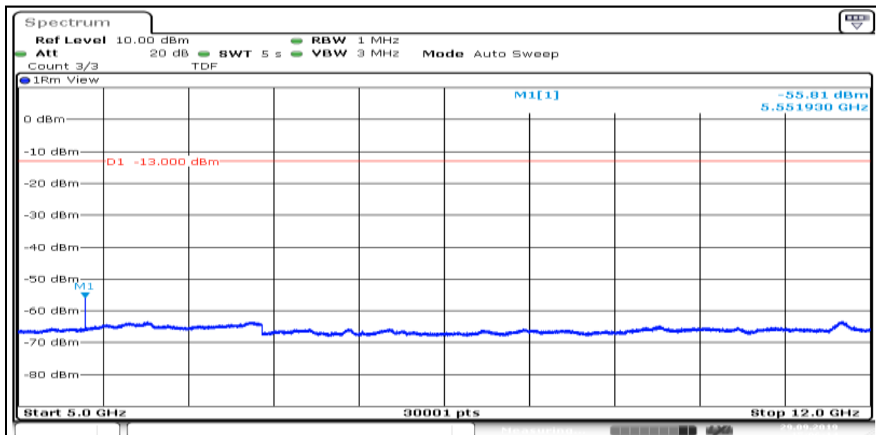
Band2_1.4MHz_16QAM_18607_6
