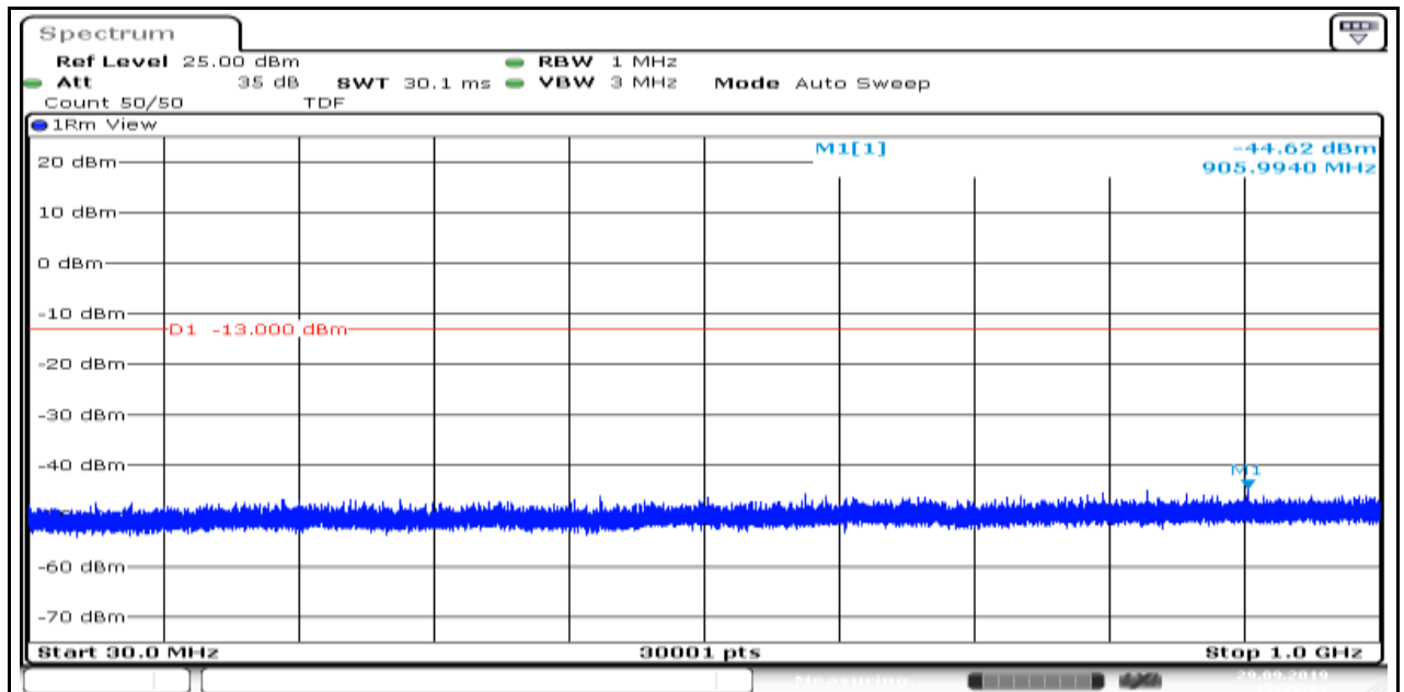
Band2_1.4MHz_16QAM_18607_6
