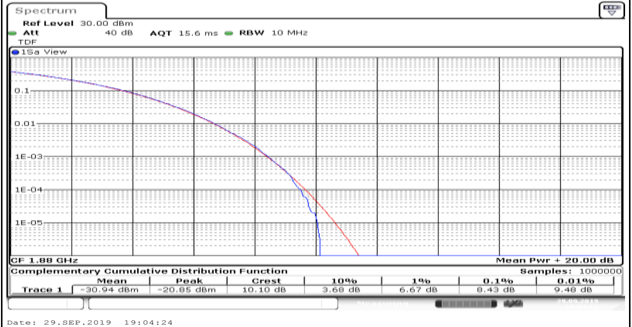
Band2_1.4MHz_QPSK_18900_6
