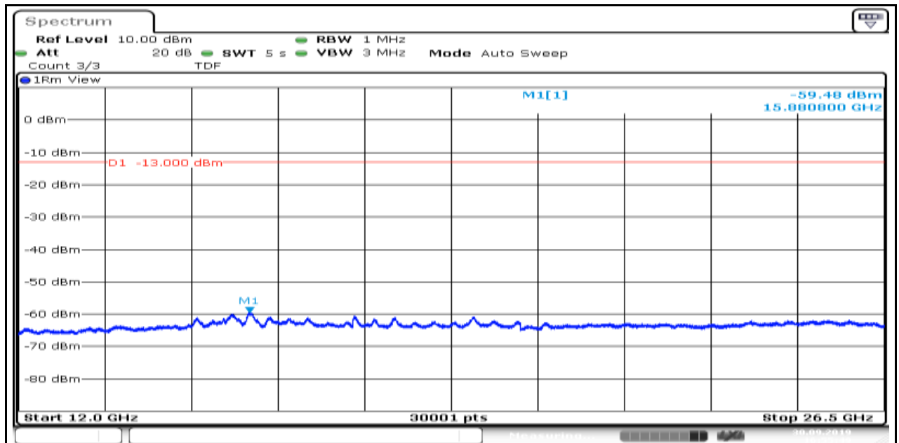
Band4_1.4MHz_QPSK_20393_1
