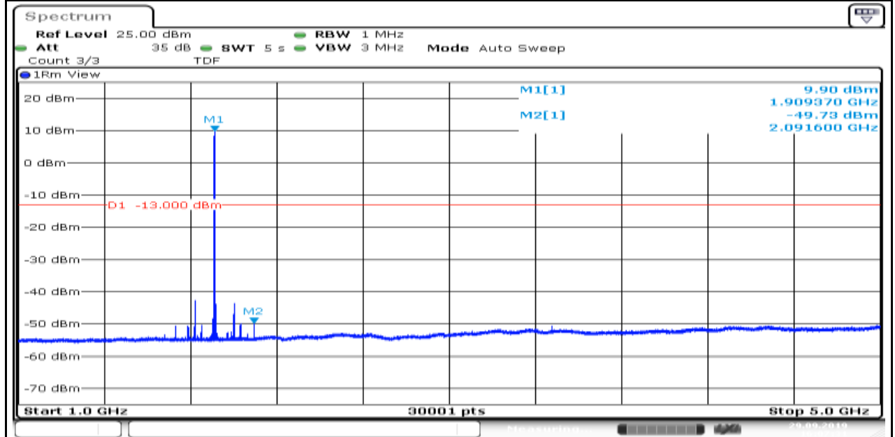
Band2_1.4MHz_16QAM_19193_6
