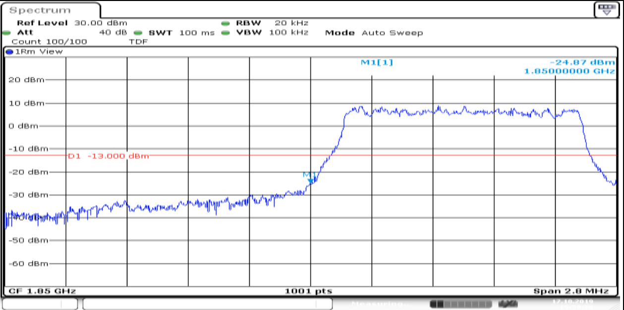
Band2_1.4MHz_16QAM_18607_6_0_Low
