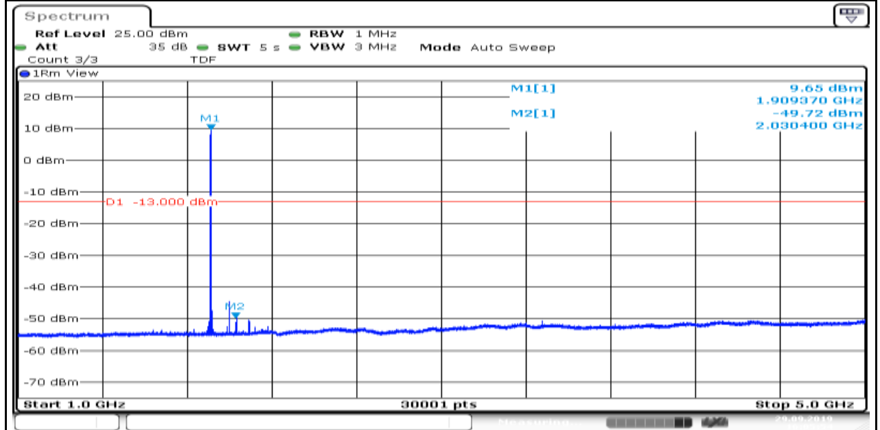
Band2_1.4MHz_QPSK_19193_6
