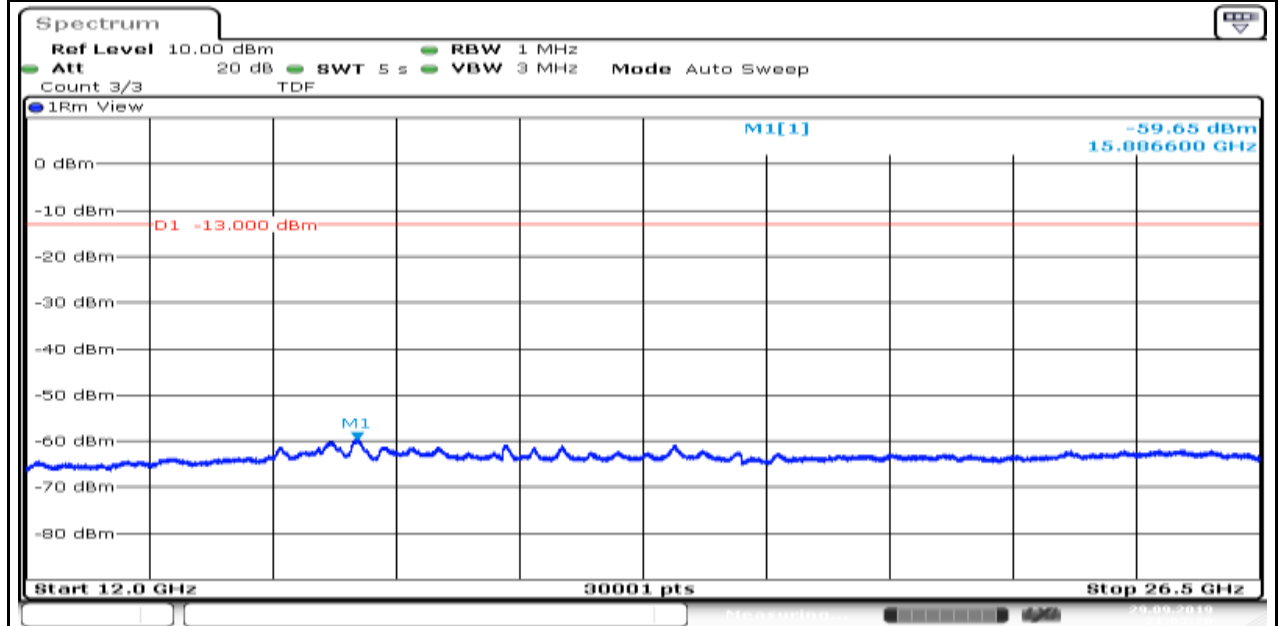
Band4_1.4MHz_16QAM_20175_6
