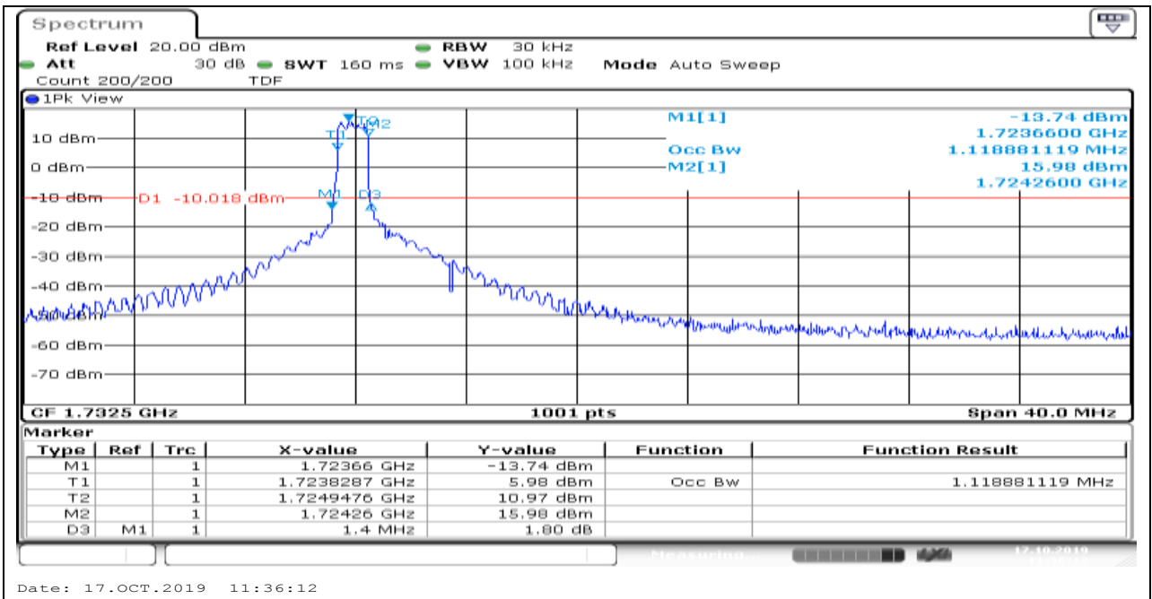
Band4_1.4MHz_QPSK_20175_6_0_Low
