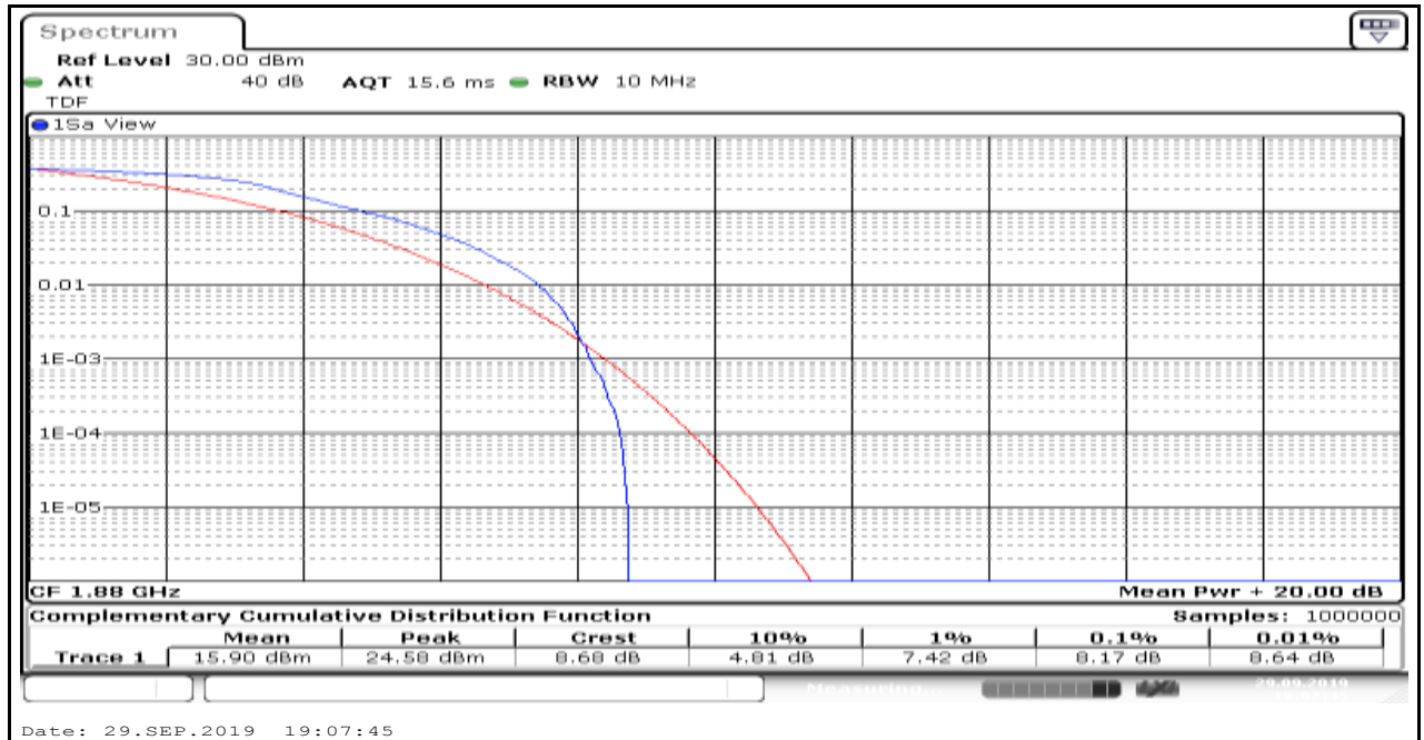
Band2_15MHz_16QAM_18900_6
