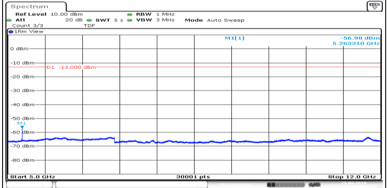
Band4_1.4MHz_QPSK_20393_5
