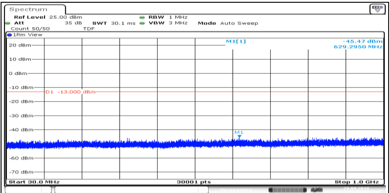
Band4_1.4MHz_16QAM_19957_6
