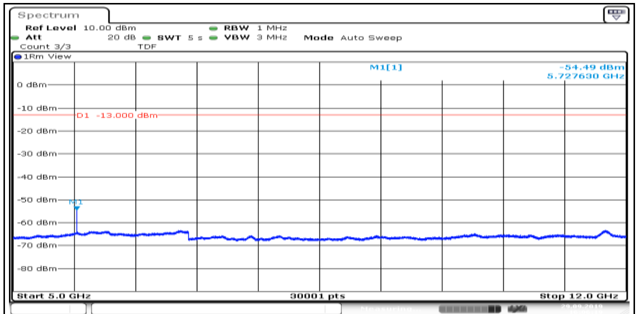
Band2_1.4MHz_QPSK_19193_6
