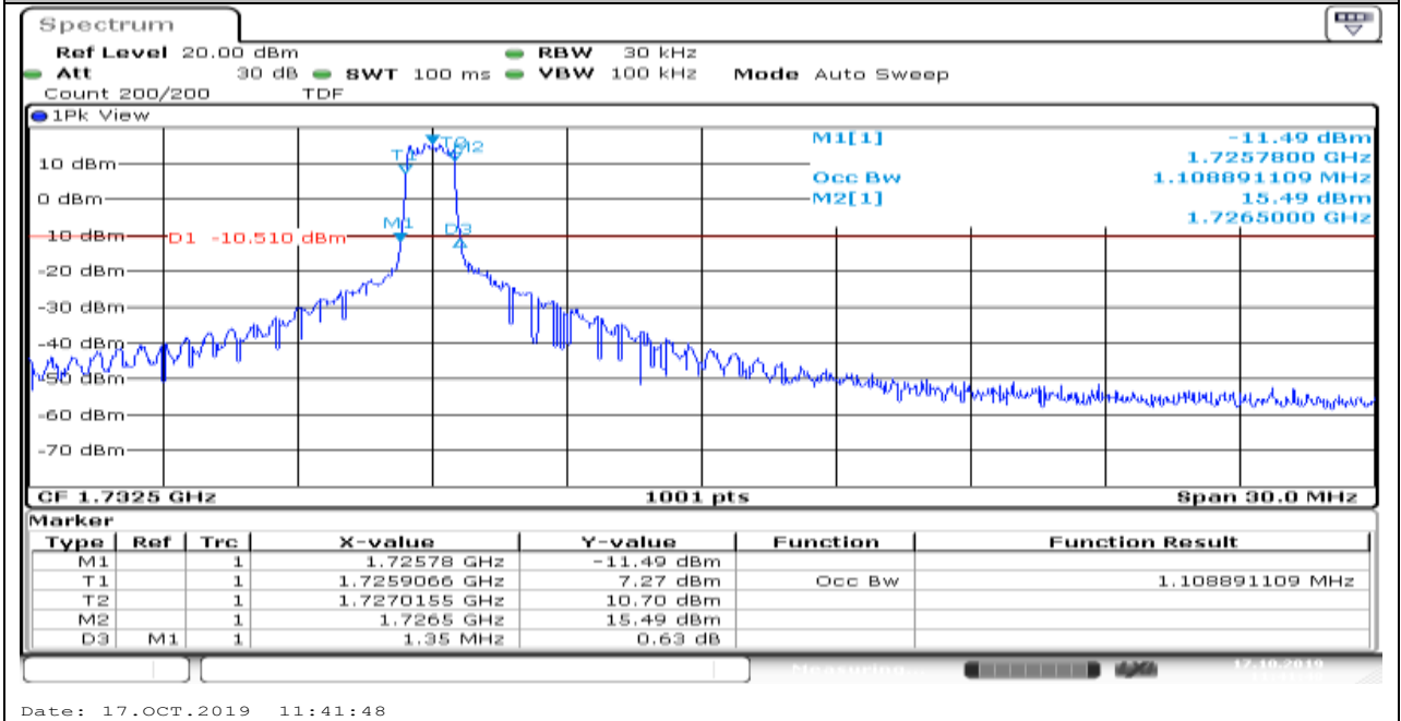
Band4_5MHz_16QAM_20175_6_0_Low
