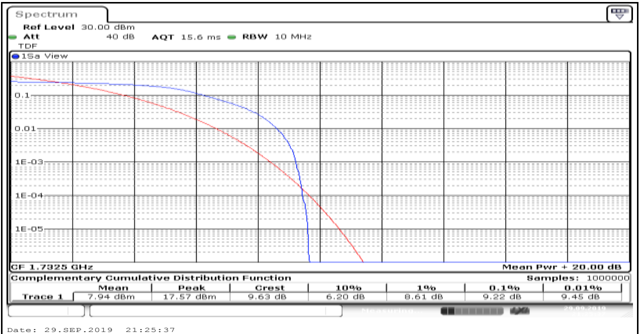
Band4_15MHz_QPSK_20175_6
