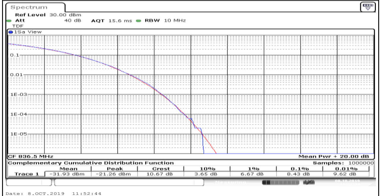
Band5_5MHz_16QAM_20525_6
