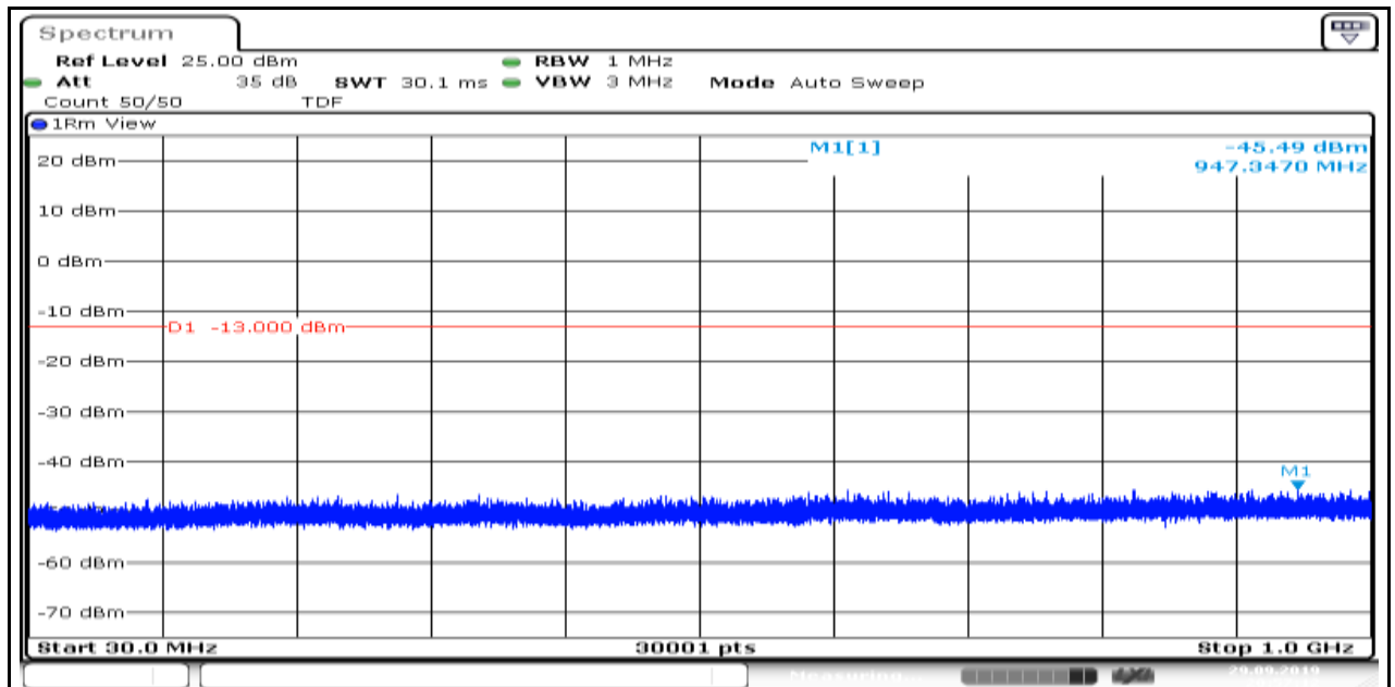
Band4_1.4MHz_QPSK_20175_6
