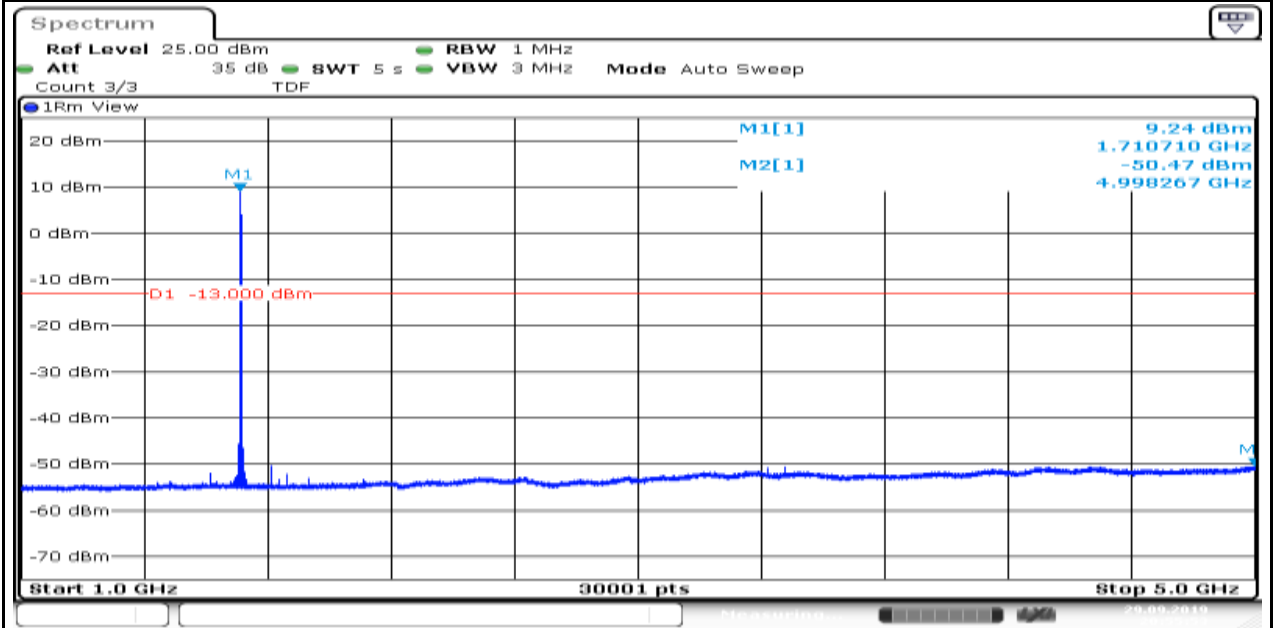
Band4_1.4MHz_16QAM_19957_6
