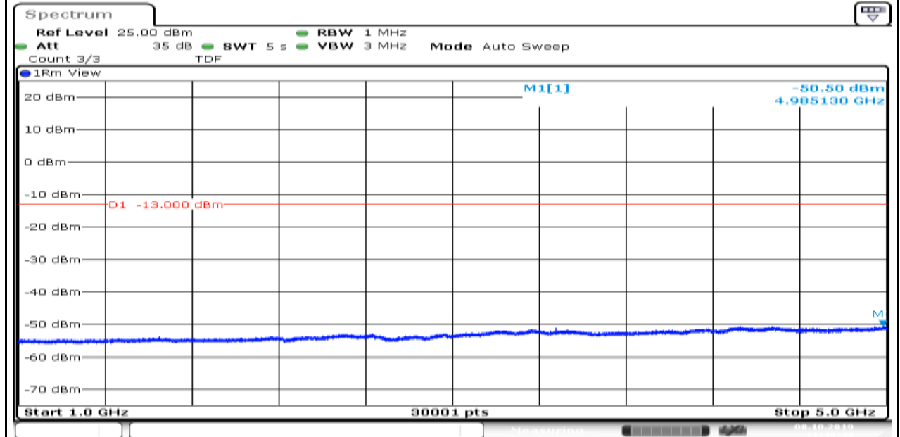
Band5_1.4MHz_QPSK_20407_6
