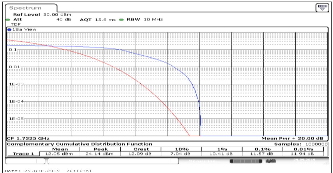
Band4_5MHz_16QAM_20175_6
