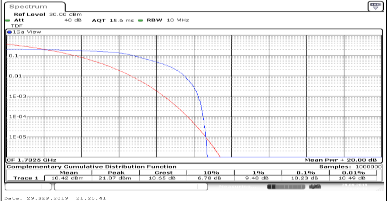
Band4_1.4MHz_16QAM_20175_6
