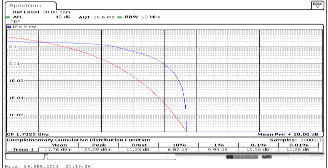
Band4_20MHz_16QAM_20175_6
