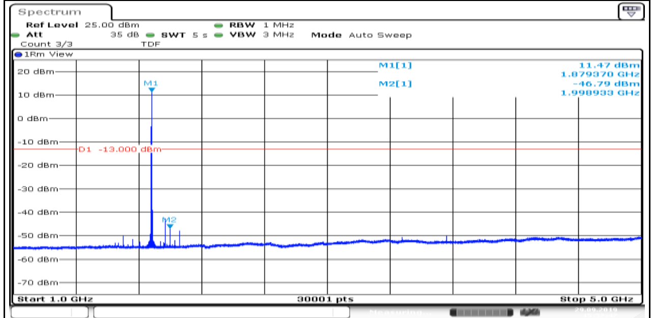
Band2_1.4MHz_16QAM_18900_1
