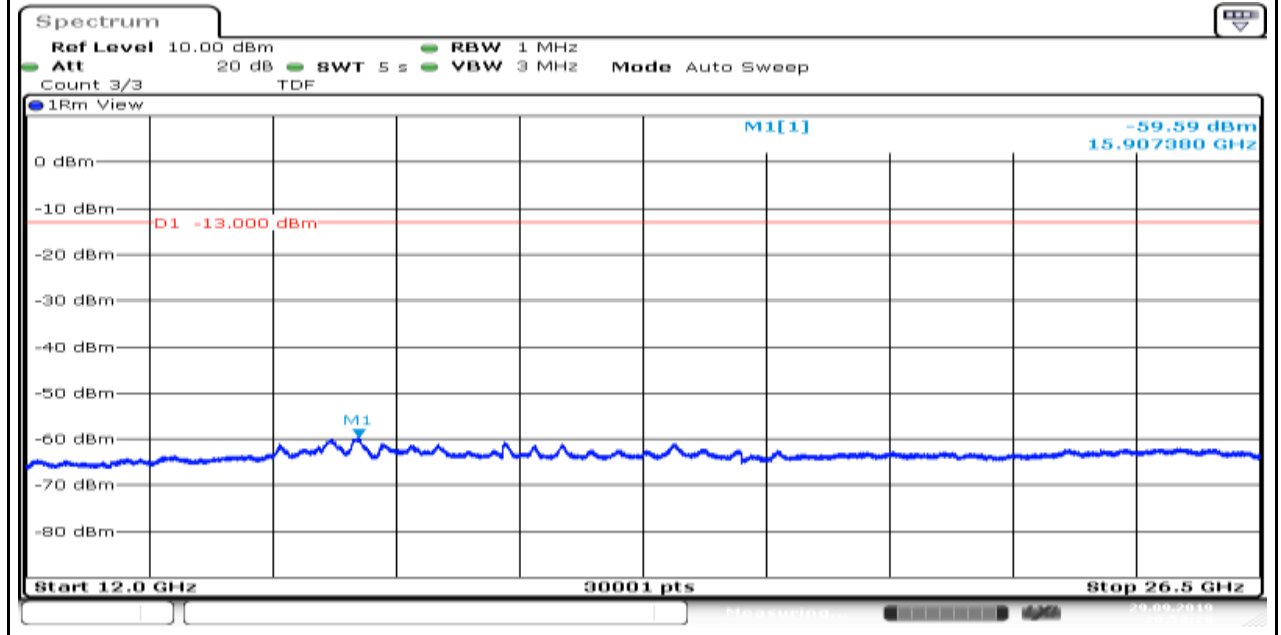
Band4_1.4MHz_QPSK_20175_1
