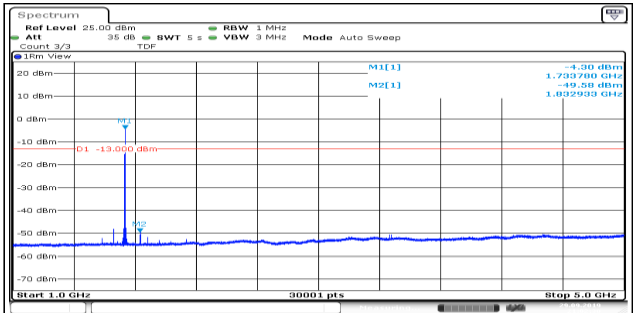
Band4_1.4MHz_16QAM_20175_6
