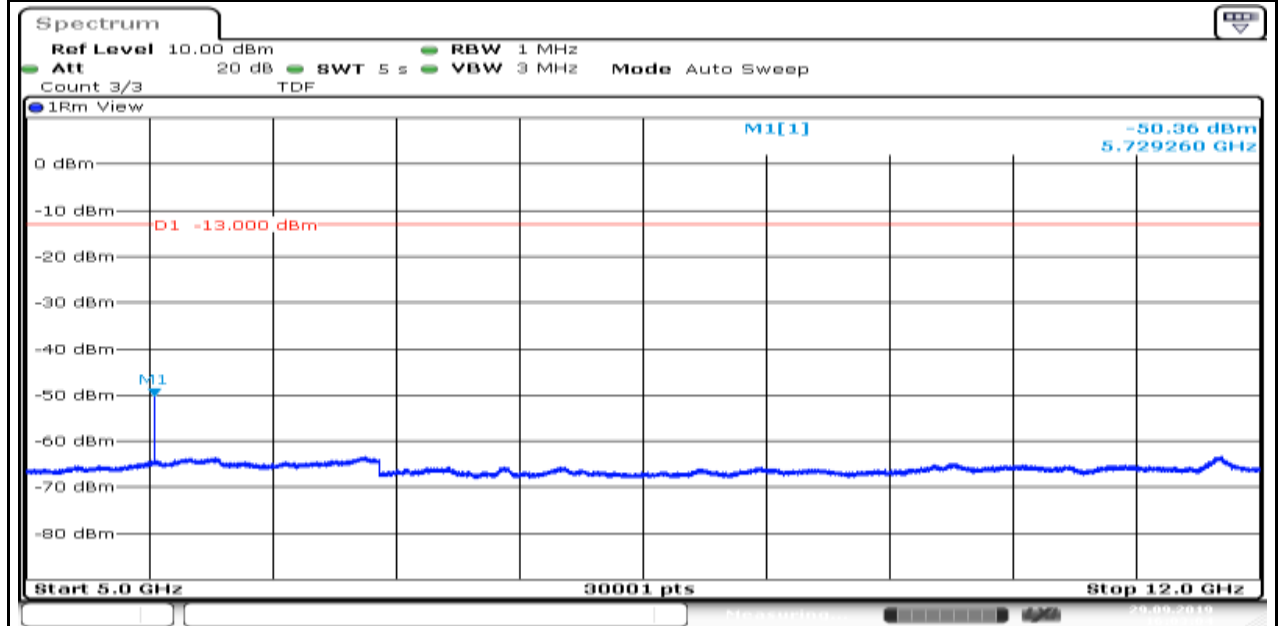
Band2_1.4MHz_QPSK_19193_1
