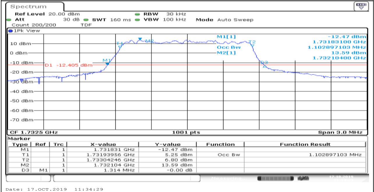
Band4_3MHz_16QAM_20175_6_0_Low
