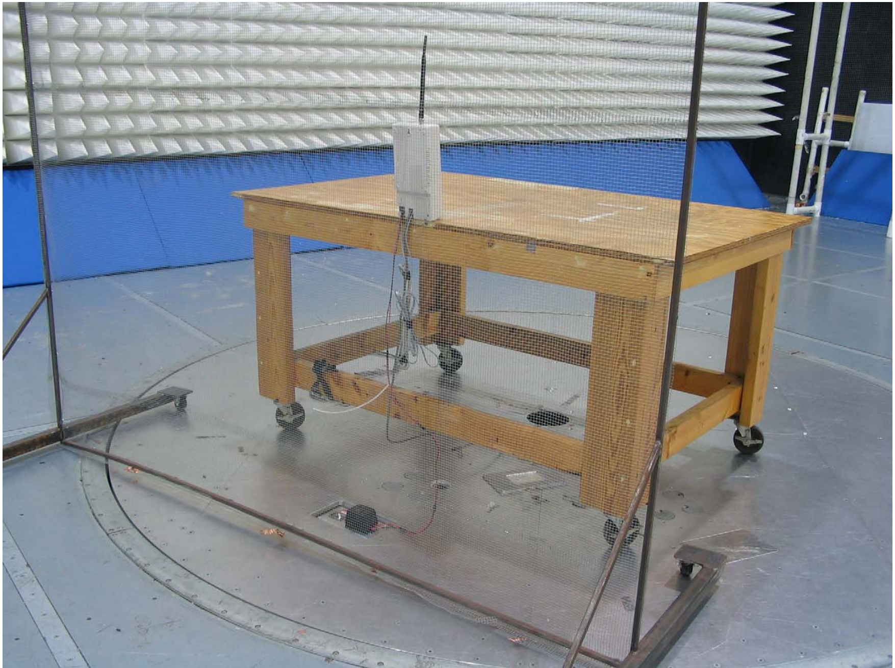
Figure 2: Conducted Emission Testing
