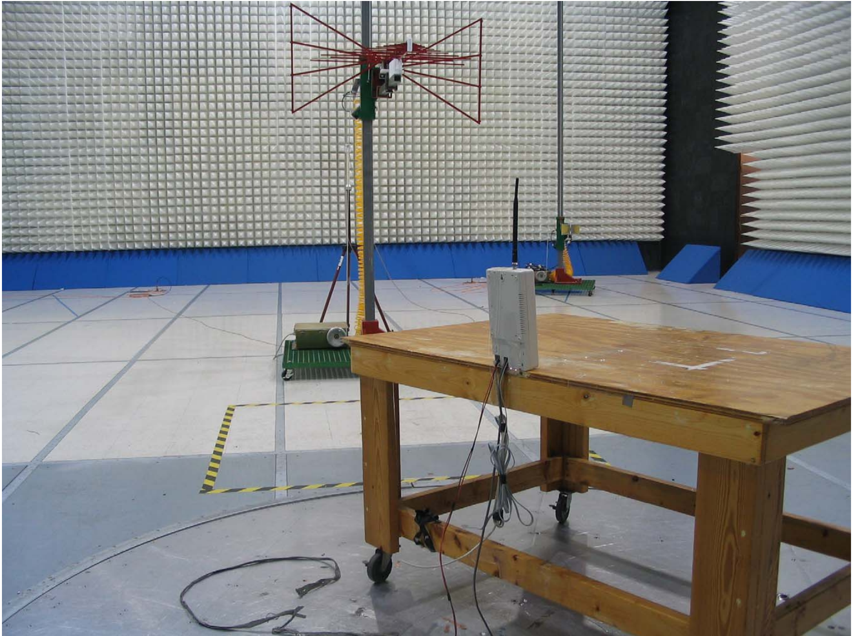
Figure 1: Radiated Emission Testing
