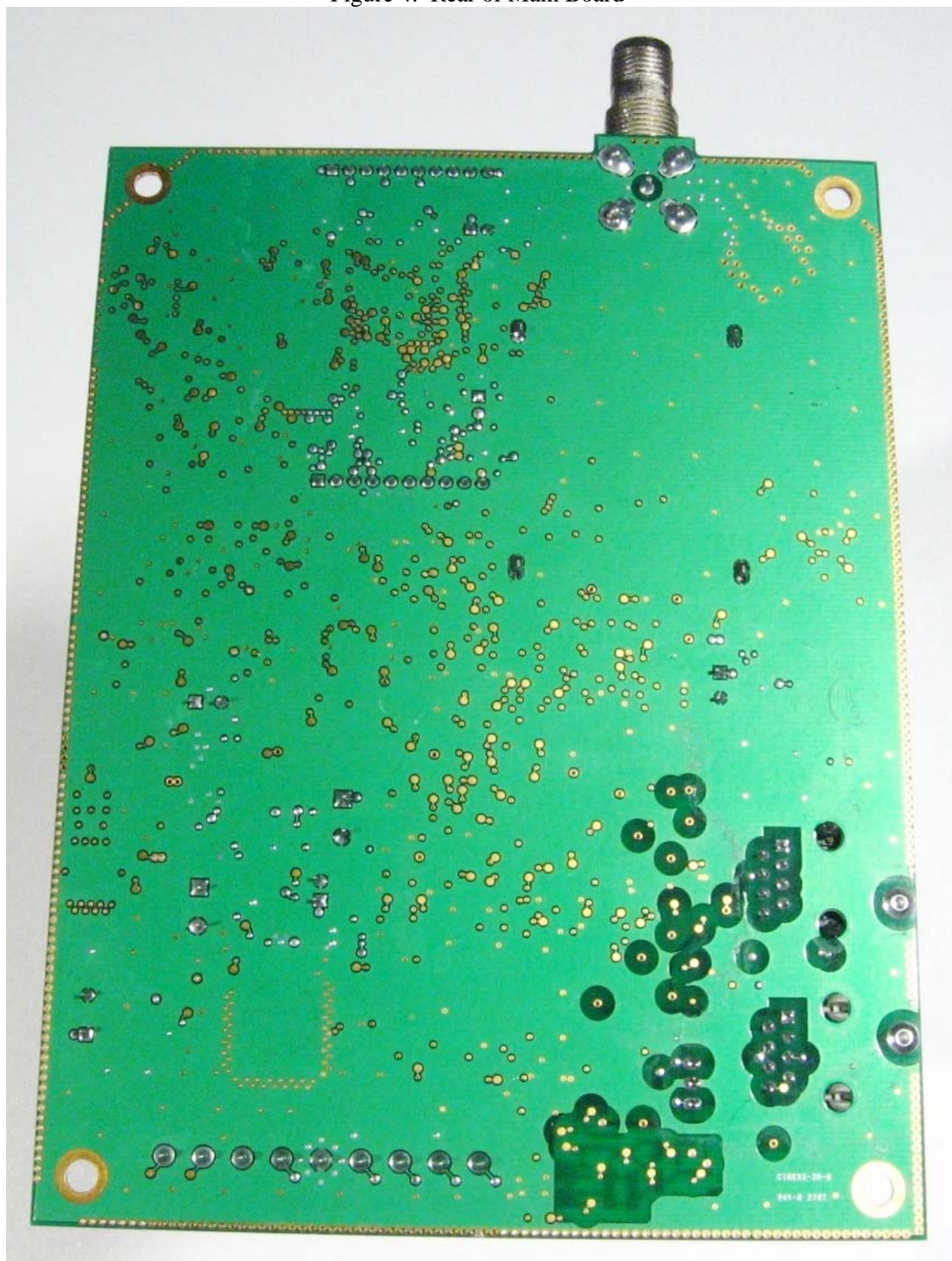
Figure 4: Rear of Main Board
