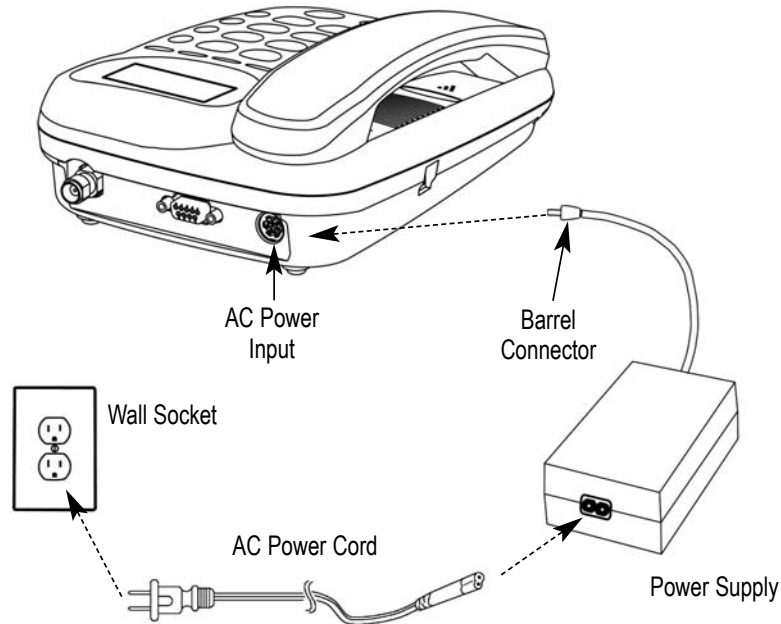
Figure 15 – SX6P AC power connection.
