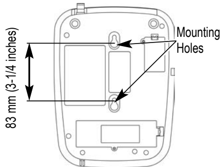
Figure 13 – SX6P mounting hooks.
