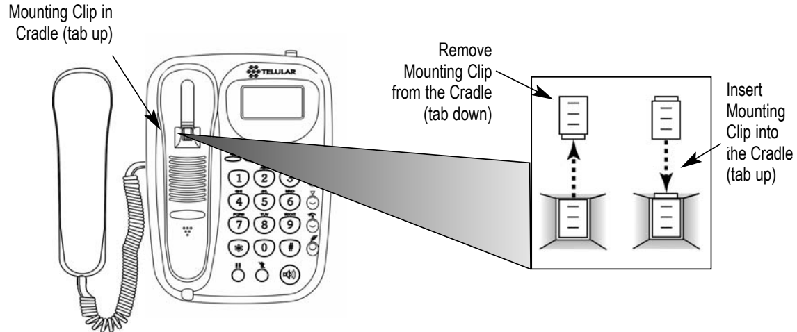
Figure 12 – Handset mounting clip for wall-mount.
