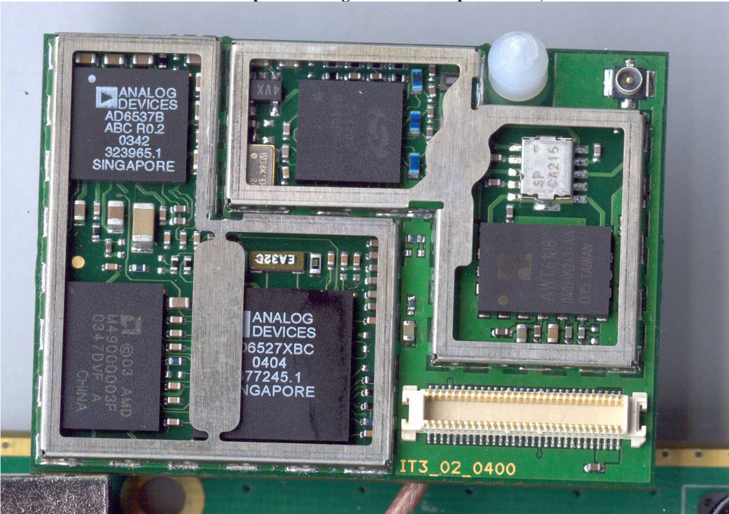
SX6P GSM 850/1900 Deskphone – Daughter Card Component Side, Shield Removed
