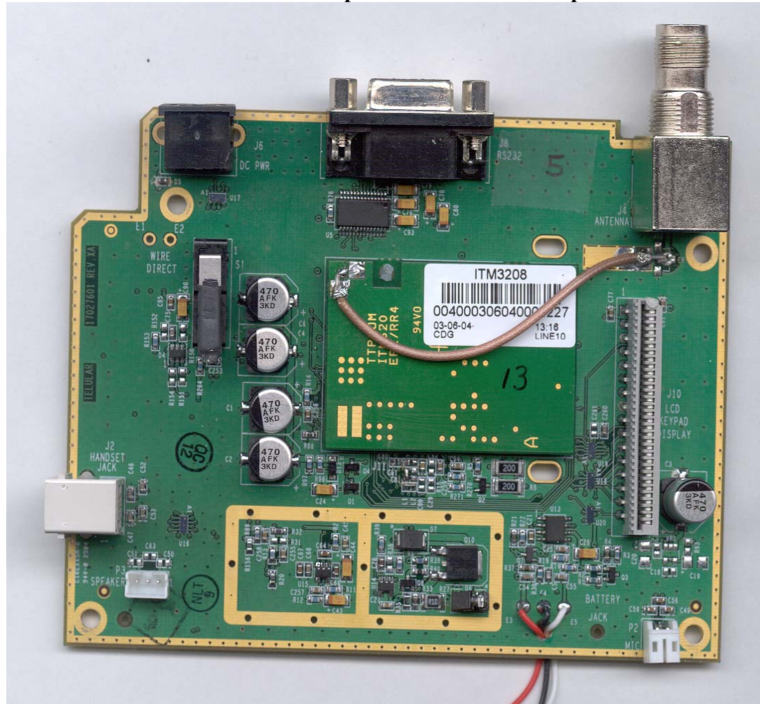
SX6P GSM 850/1900 Deskphone – RF Board Component Side
