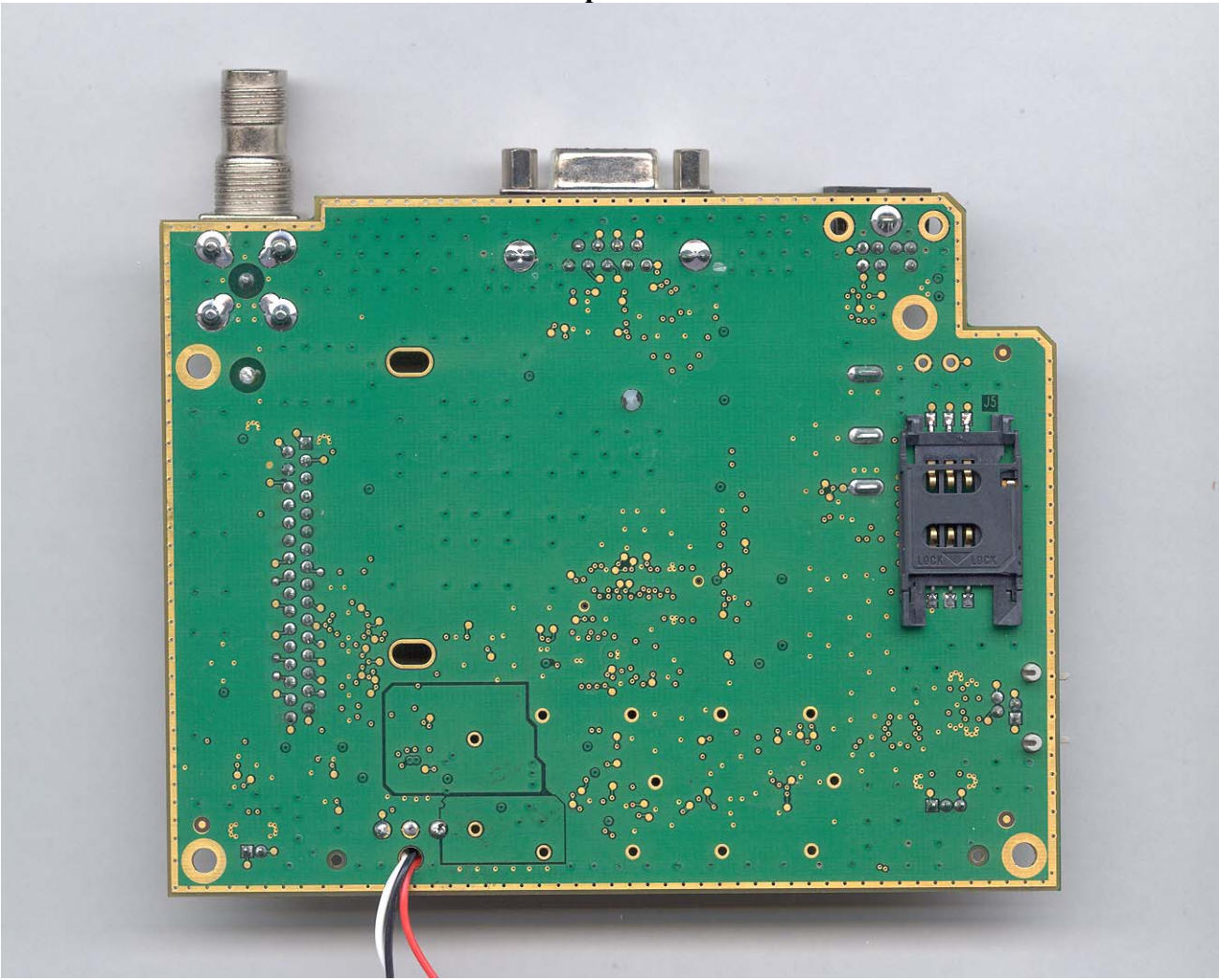
SX6P GSM 850/1900 Deskphone – RF Board Solder Side
