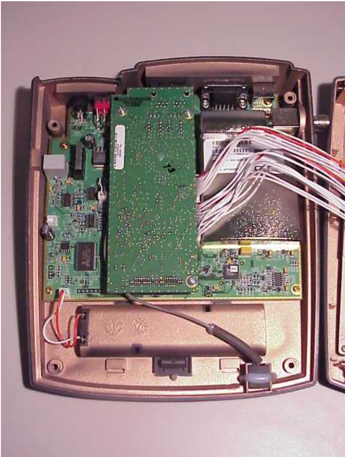
Figure 3: Bottom cover with circuit boards installed – SX5D
