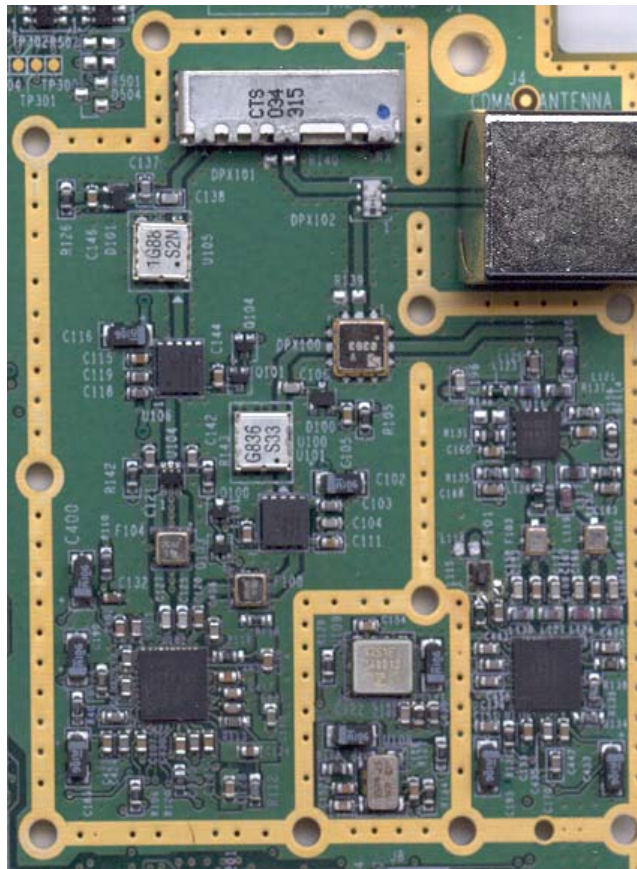
Figure 5: Main Board Close up of Covered Area
