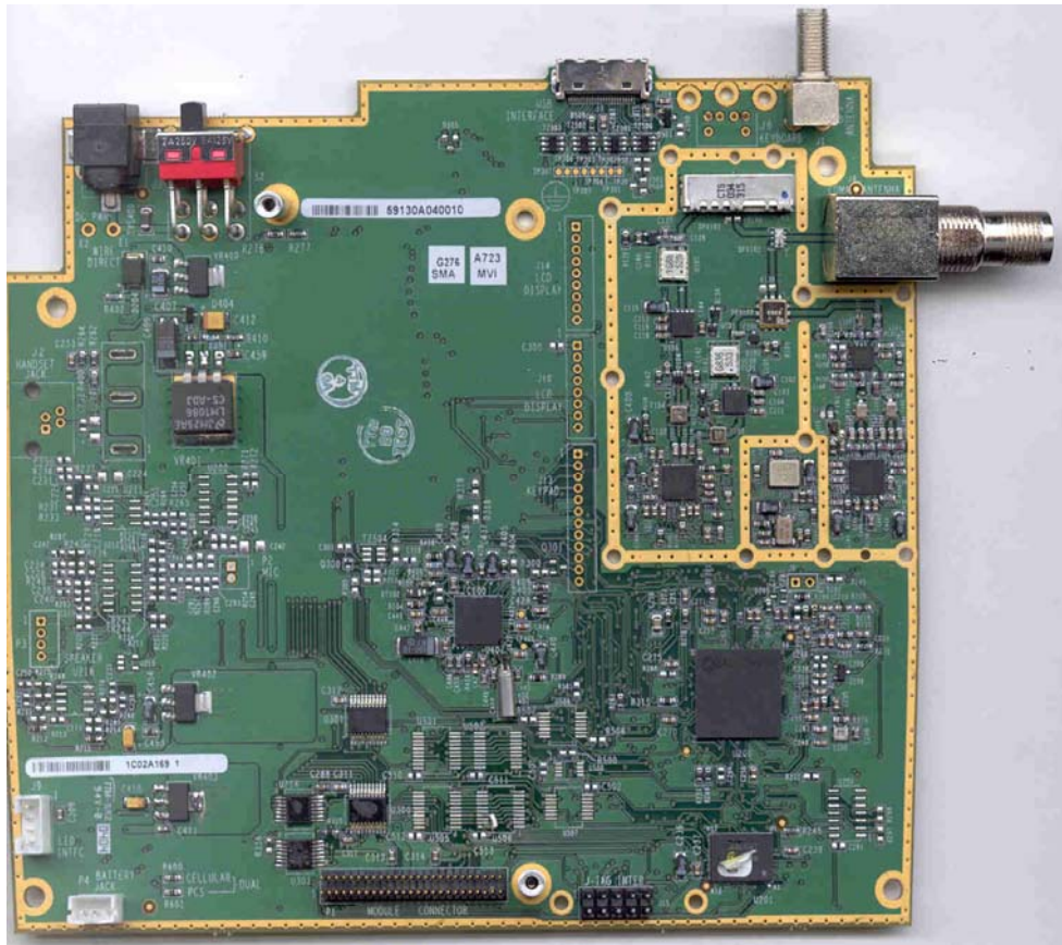
Figure 4: Main Board with Covered Area Exposed
