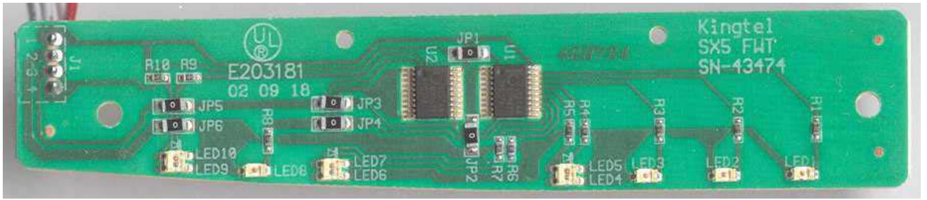
Figure 8: DC Power Board Front
