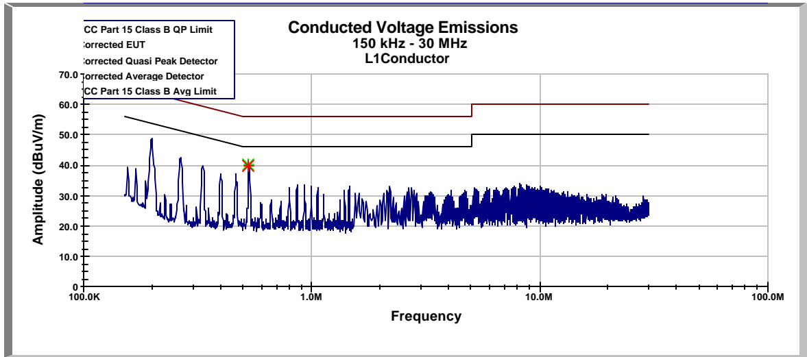
Figure 9-3: FCC §15.107 and §15.207 power line conducted emissions (Line 1 on the CDMA800 Phone)
