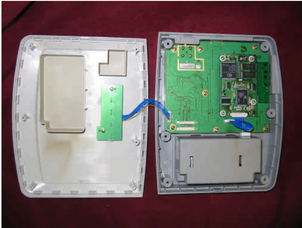
Main Circuit Board
