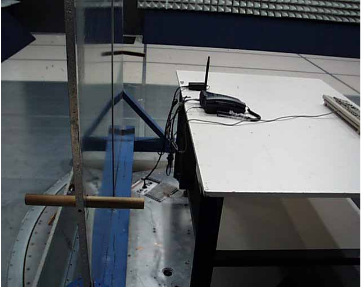
Figure 2: Conducted emissions, rear view
