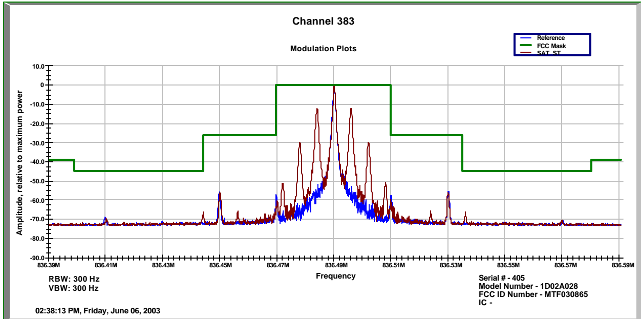
Figure 7-2: Occupied bandwidth – SAT and ST
