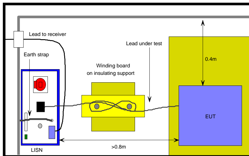
Arrangement of the EUT
