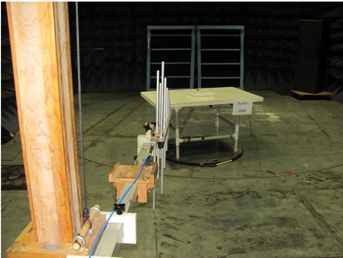
200 to 1000 MHz
