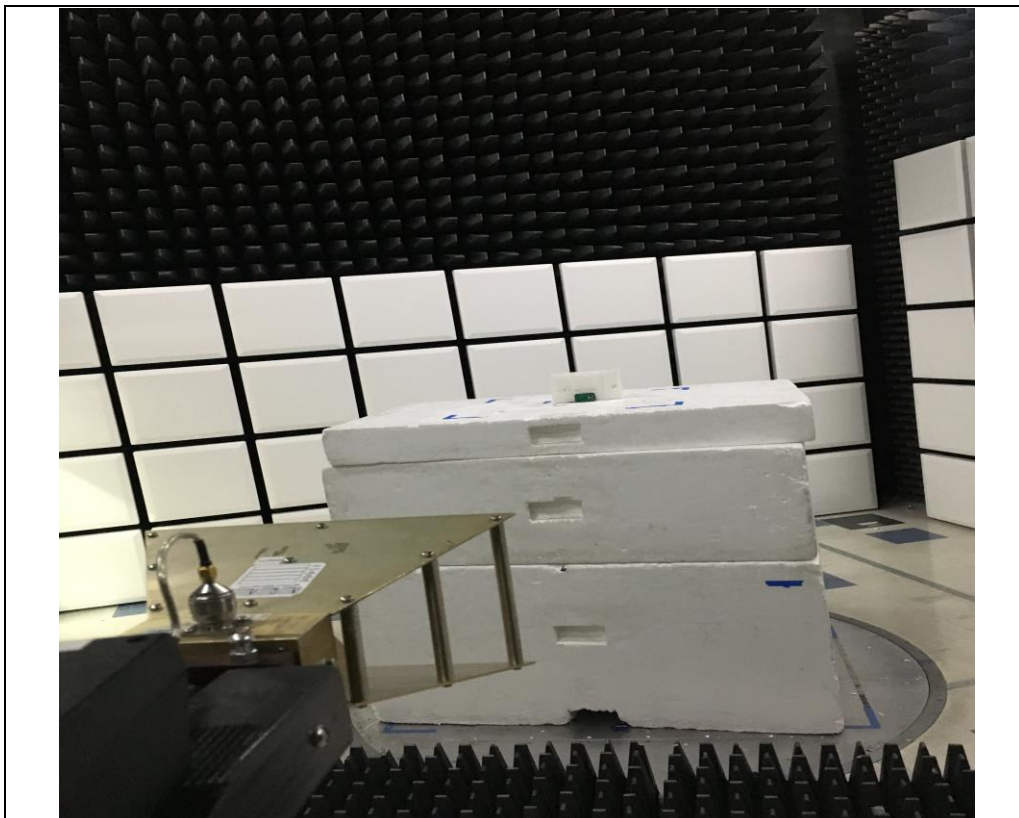
RF Radiated #2
