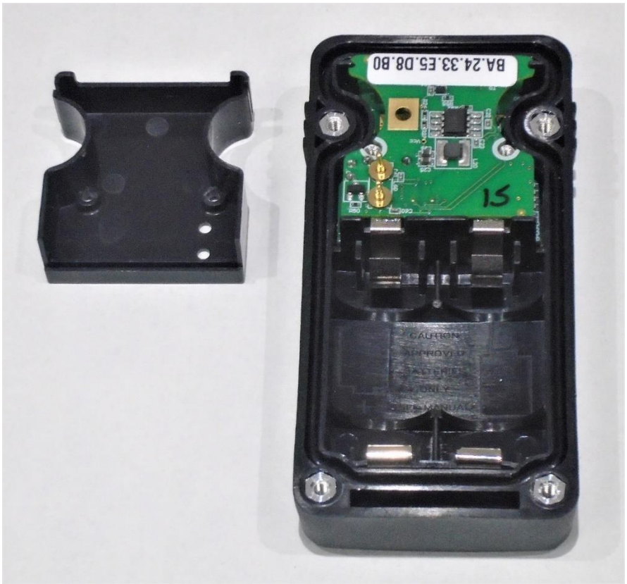
Interior with both PCBs Installed.
